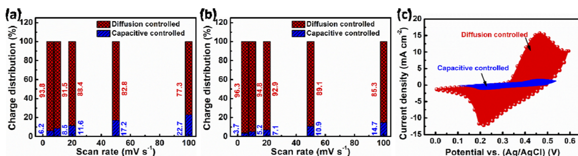
Fig. 6 Diffusion- and capacitive-controlled charge storage contributions in the (a) bare \text{NiCo}_2\text{O}_4 and (b) \text{NiCo}_2\text{O}_4@\text{CuS} composite electrodes at varying scan rates. (c) Capacitive and diffusion-controlled charge storage contribution breakdown in the \text{NiCo}_2\text{O}_4@\text{CuS} composite electrode at 10 \text{ mV s}^{-1} .
