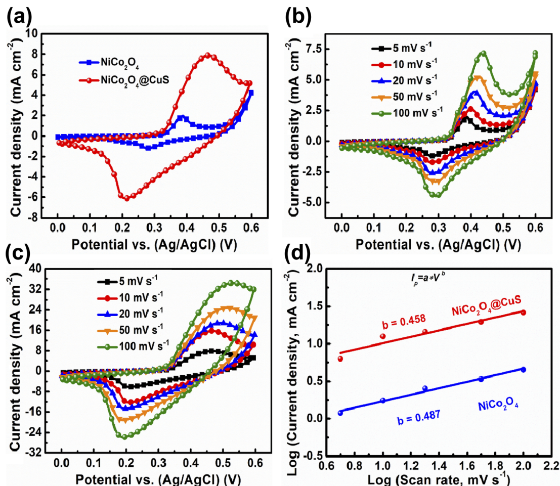
Fig. 5 (a) Comparative CV curves of the as-prepared electrodes at 5 \text{ mV s}^{-1} . CV plots of (b) bare \text{NiCo}_2\text{O}_4 and (c) \text{NiCo}_2\text{O}_4@\text{CuS} composite electrode. (d) Relationship between the \log(i_p) and \log(v) .
