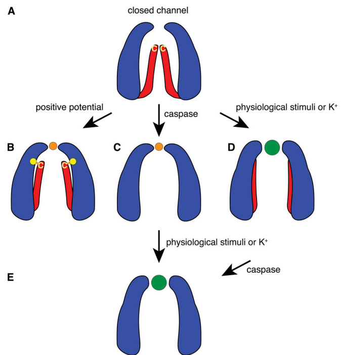
Figure 5. Activation mechanisms of Panx1 channels. (A) Based on the presently available structural and functional data, we hypothesize that the closed channel exhibits the external restriction of ~9 Å and that the C termini reach deep into the pore, occluding it. (B) Depolarization dislocates the C termini, so that the channel pore diameter equals or exceeds that of the external restriction and exposes the terminal cysteine (yellow C) to thiol reagents. The yellow dot indicates the position of Panx1F54 which, when mutated to a cysteine, can be disulfide bonded with the terminal cysteine (Sandilos et al., 2012). In this configuration, the external restriction limits entry by size and selects for chloride (orange dot) over other ions. (C) Cleavage of Panx1 at position 378 removes the “pore gate,” rendering the channel constitutively active. However, as indicated by the published cryo-EM data, caspase cleavage does not affect the external constriction, leaving a chloride-selective channel. (D) Various physiological stimuli initiate a gating mechanism at the external restriction, widening it to accept ATP (green dot) and other molecules in this size range. (E) This mechanism also may move charged amino acids within the external constriction, with the consequence that charge selectivity is attenuated. In the case of K + stimulation, the terminal cysteine is no further reactive to thiol reagents, while engineered cysteines at the external end of the pore still are. Whether this terminal cysteine concealment also applies to the physiological stimuli remains to be determined. Cleavage of the C terminus by caspase “super stimulates” the channel and irreversibly seals the apoptotic fate of the cell.
