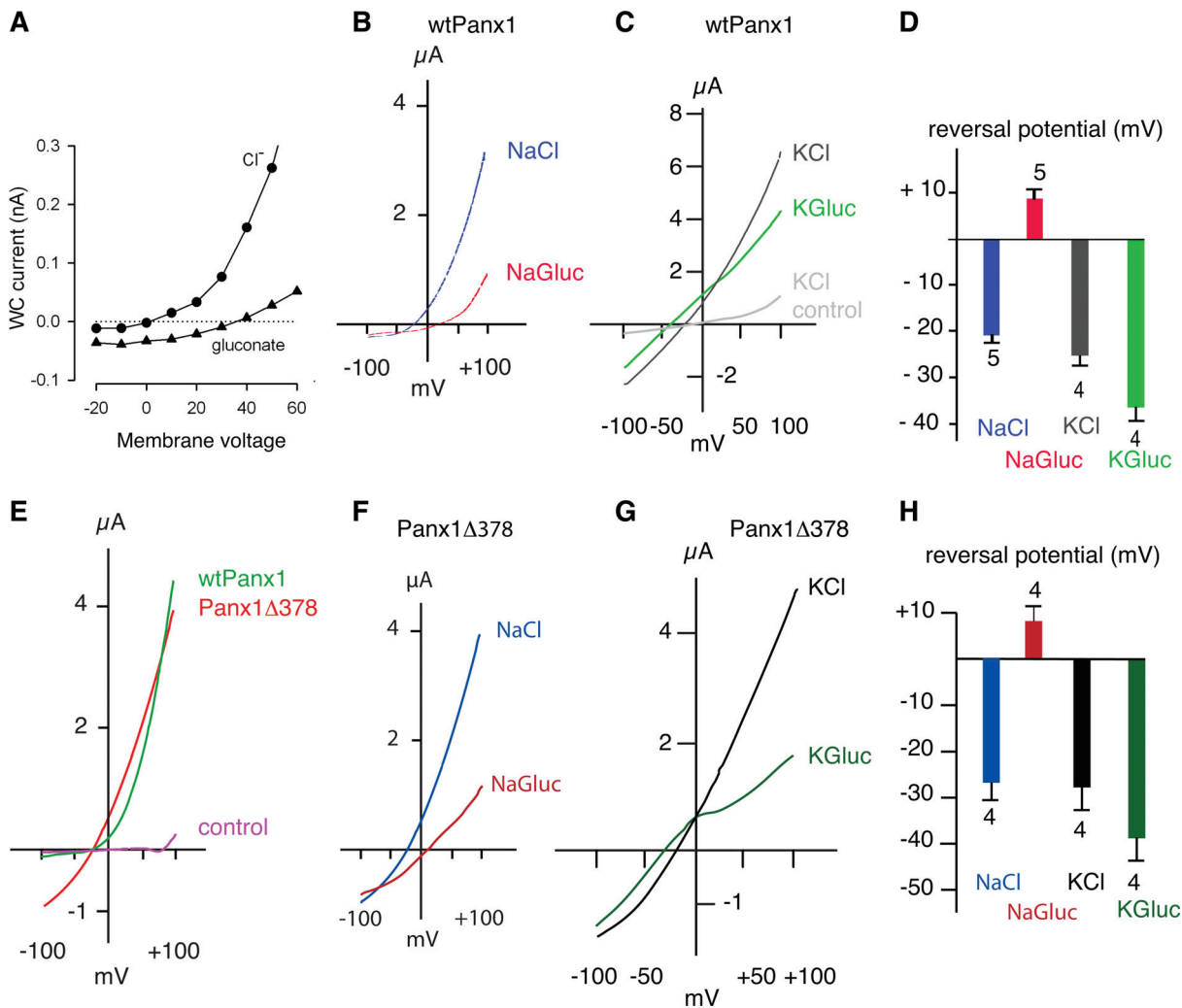
Figure 3. Current–voltage relations of mouse WT Panx1 and Panx1 \Delta 378. (A) Replacing extracellular Cl - by gluconate - in a voltage step protocol applied to HEK cells expressing Panx1 exogenously attenuated the membrane currents and shifted the reversal potential to a positive potential. Adapted with permission from Journal of Cell Science (Romanov et al., 2012). (B) Similarly, in oocytes expressing Panx1 exogenously, replacement of Cl - by gluconate - (NaGluc) resulted in a shift of the reversal potential to positive values and an attenuation of the currents induced by a voltage ramp from -100 to +100 mV. (C) Voltage ramp–induced currents of wtPanx1-expressing oocytes in KCl solution (black trace) were substantially larger than the currents in uninjected control cells under identical conditions (gray trace). Replacing Cl - by gluconate - in the bath solution of the same oocyte resulted in attenuation of the currents and a shift of the reversal potential to more negative potential (green trace). (D) Quantitative analysis of reversal potentials after anion replacement shows a shift from positive to negative potentials with K + as the extracellular cation. Means \pm SE; n = 5 (wtPanx1). (E) Voltage ramp–induced membrane currents of WT Panx1 channels (green trace) and of channels formed by the truncation mutant Panx1 \Delta 378, where C-terminal amino acids after aspartate 378 are deleted. Uninjected oocytes served as control (magenta trace). Because Panx1 \Delta 378-expressing cells had a short life span, mRNA was injected 80 \times diluted as compared with WT, and measurements were performed in a 24-h window. Thus, the current amplitudes of WT Panx1 and Panx1 \Delta 378 cannot be compared. In contrast to WT Panx1 channels, those formed by Panx1 \Delta 378 were active over a wide voltage range, yet currents through both types of channels reversed at the same membrane potential. (F) Similar to WT Panx1, currents through Panx1 \Delta 378 channels reversed at negative membrane potential with extracellular chloride (blue trace) and at positive potential with gluconate solution (red trace). (G) Similar to WT Panx1 channels, replacement of chloride by gluconate ions resulted in the currents reversing at negative potentials when Panx1 \Delta 378-expressing cells were exposed to high extracellular K + . (H) Quantitative analysis of reversal potentials of membrane currents carried by Panx1 \Delta 378 after anion replacement shows a shift from positive to negative potentials with K + as the extracellular cation. Means \pm SE; n = 4. (B–H) Data from Wang and Dahl (2018).
