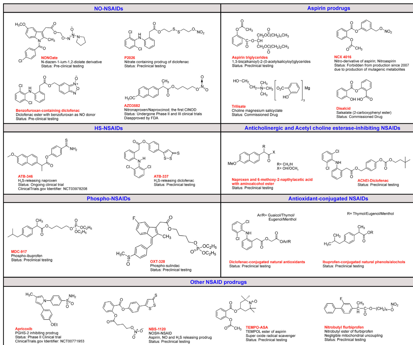
Fig. 6. Structural representation of some NSAID prodrugs.
