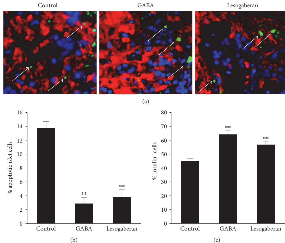
FIGURE 3: Oral lesogaberan protects human islet \beta -cells from apoptosis in islet grafts in mice. Diabetic NOD/scid mice were implanted with human islets and treated with plain water or water containing lesogaberan (0.08 mg/ml) or GABA (6 mg/ml) for 48 h. The percentages of apoptotic islet cells and islet \beta -cells in total human islet cells were determined by TUNEL assay and costaining with anti-insulin as well as DAPI. At least 2000 human islet cells in 10 fields (magnification \times 400 ) from individual grafts were counted. Data are representative image or expressed as the mean \% \pm SEM for each group of mice ( n = 5 - 7 ) from three separate experiments. (a) A representative image with white arrows indicating TUNEL + cells (green for TUNEL + , red for anti-insulin + , and light blue for DAPI staining). (b) Percent apoptotic islet cells and (c) percent insulin + islet cells. ** p < 0.01 versus the control.
