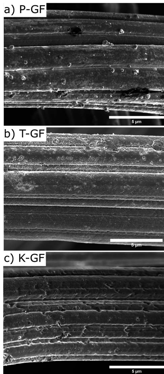
Fig. 3 SEM images displaying the surface morphology of (a) P-GF electrode, (b) T-GF electrode and (c) K-GF electrode.
