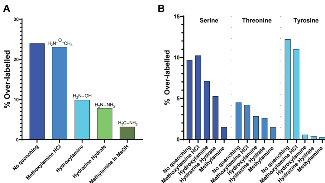
FIG. 3. Screening of aminolysis reagents. A, bar chart showing the percentage of the intensity attributable to peptides containing at least one overlabelled residue after treatment with 50% acetonitrile (control) or 0.3 M of each: methoxylamine, hydroxylamine, hydrazine hydrate, and methylamine. B, a bar chart showing the percentage of overlabelled peptide intensity by ester type after each treatment.
