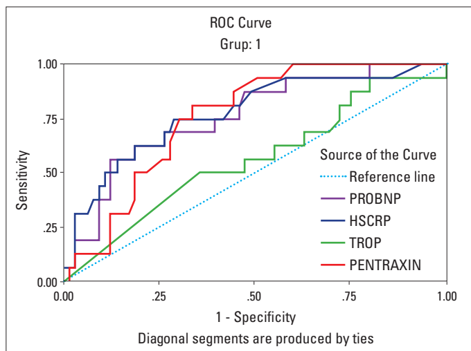
Figure 1. The discriminatory value of PTX3 levels for long-term cardiovascular mortality in STEMI group by receiver operating (ROC) curve analysis
