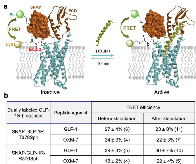
Fig. 5 (a) Scheme for inter-domain movement upon ligand stimulation to activate the with the dually fluorescently labelled GLP-1R monitored by FRET. (b) Measured FRET efficiencies before and after ligand stimulation. The numbers in parenthesis represent the individual cells used in acceptor photobleaching to determine FRET efficiency as reported in mean \pm standard deviation. Representative confocal micrographs used for determining FRET efficiencies are shown in the ESI,† Fig. S6–S9.
