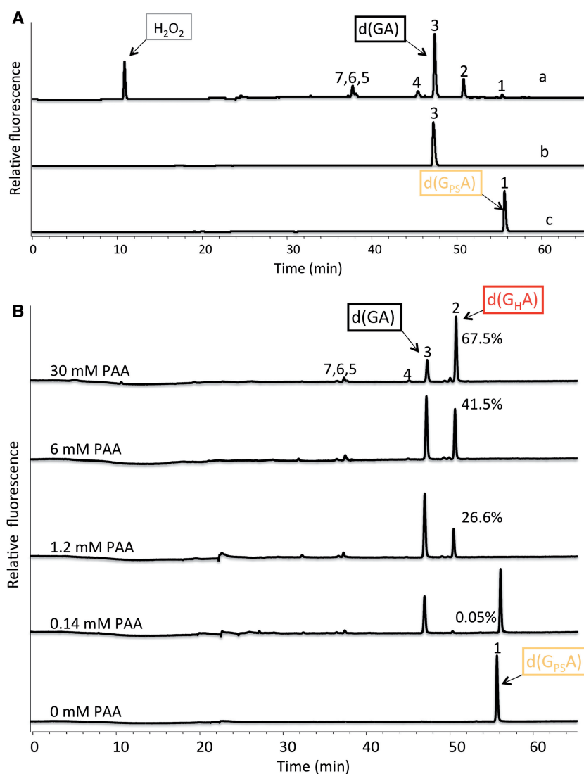
Figure 2. PT dinucleotide is oxidized by H_2O_2 and PAA. (A) Conversion of d(G PS A) to d(GA) by H_2O_2 . d(G PS A) was incubated with (110 mM) H_2O_2 , generating reaction products 2–7 (a). The main product is 3. d(GA) (b) and d(G PS A) (c) were run as control. Note the remaining H_2O_2 peak can be observed. (B) HPLC traces showing the conversion of PT to H-phosphonate linkage by increasing concentrations of per-acetic acid (PAA). Note the amount of reaction product 2, H-phosphonate dinucleotide [d(G H A)], increased corresponding to increasing concentration of PAA. At 30 mM concentration of PAA, d(G PS A) is converted mainly to d(G H A) (~67.5% of reaction products under the reaction condition). (C) High resolution mass spectrum analysis of H-phosphonate dinucleotides. Mass fragmentations of d(G PS A) (1), d(G H A) (2) and d(GA) (3). Characteristic mass peaks m/z = 348 , 316 and 332, indicating the linkages of PT, H-phosphonate and phosphodiester were marked. Fragmentation peaks corresponding to G ( m/z = 152 ) and A ( m/z = 136 ) were also indicated. (D) HPLC traces showing the hydrolyzed products of synthesized d(G H A) standard and the lyophilized d(G H A) generated by oxidizing d(G PS A) using PAA. Note, after release from the synthesizing column by ammonium hydroxide, all d(G H A) was hydrolyzed, generating products 4–7 mainly. Peak 3 was barely detectable. d(G PS A) oxidized by PAA generated d(GA) (peak 3) as a main product. For mass fragmentation of peak 4–7 (see Supplementary Figure S2S).
