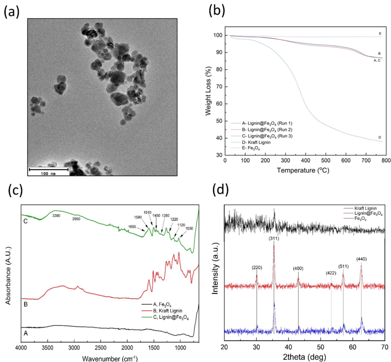
Fig. 1 Characterizations of neat Fe 3 O 4 , kraft lignin, and lignin@Fe 3 O 4 . (a) TEM images of lignin@Fe 3 O 4 ; (b) TGA results for lignin@Fe 3 O 4 (A–C), KL (D), and neat Fe 3 O 4 nanoparticles (E); (c) FT-IR spectra of neat Fe 3 O 4 , kraft lignin (KL), and lignin@Fe 3 O 4 nanoparticles; (d) XRD spectra for kraft lignin (black), lignin@Fe 3 O 4 (red), and neat Fe 3 O 4 (blue) powder samples. The numbers in the parenthesis represent the Miller indices at each of the Bragg reflections (peaks).
