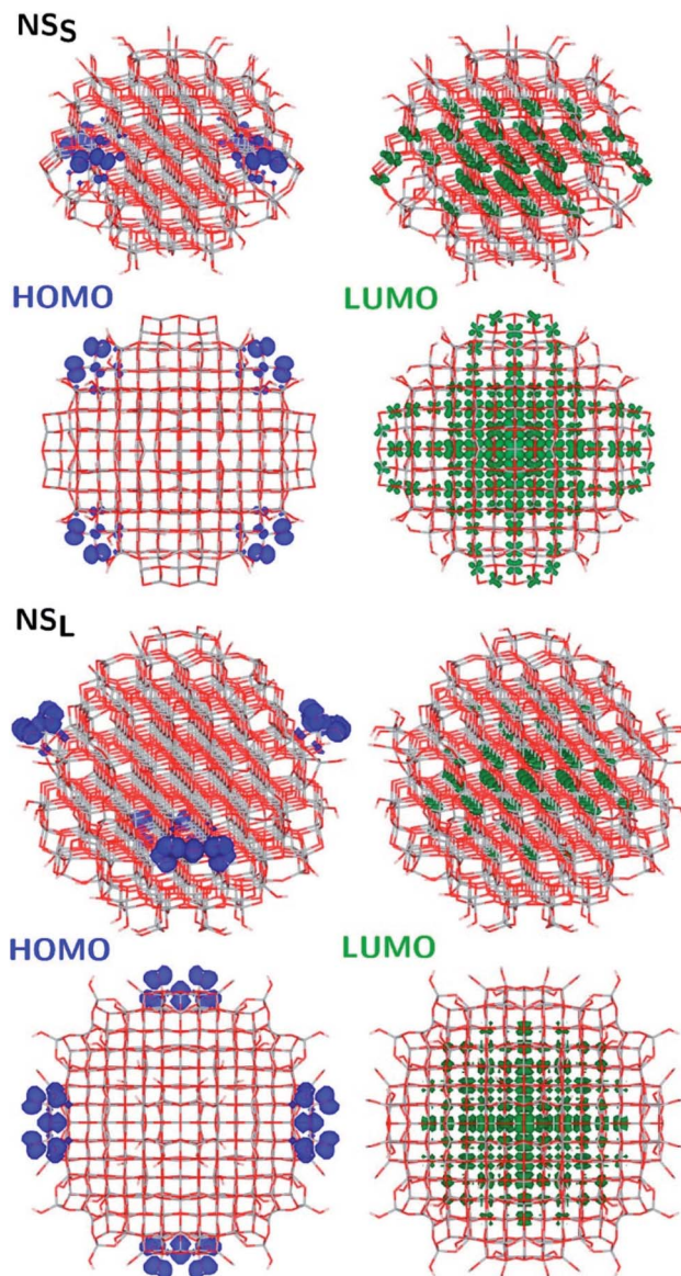
Fig. 11 Side (upper) and top (lower) views of the electronic density plots of the frontier orbitals of \text{NS}_5 and \text{NS}_L (isosurface = 5 \times 10^{-4} au, except for HOMO, for which isosurface = 1 \times 10^{-3} au). Reprinted with permission from G. Fazio, L. Ferrighi and C. Di Valentin, J. Phys. Chem. C , 2015, 119 , 20735–20746. Copyright 2015 American Chemical Society.
