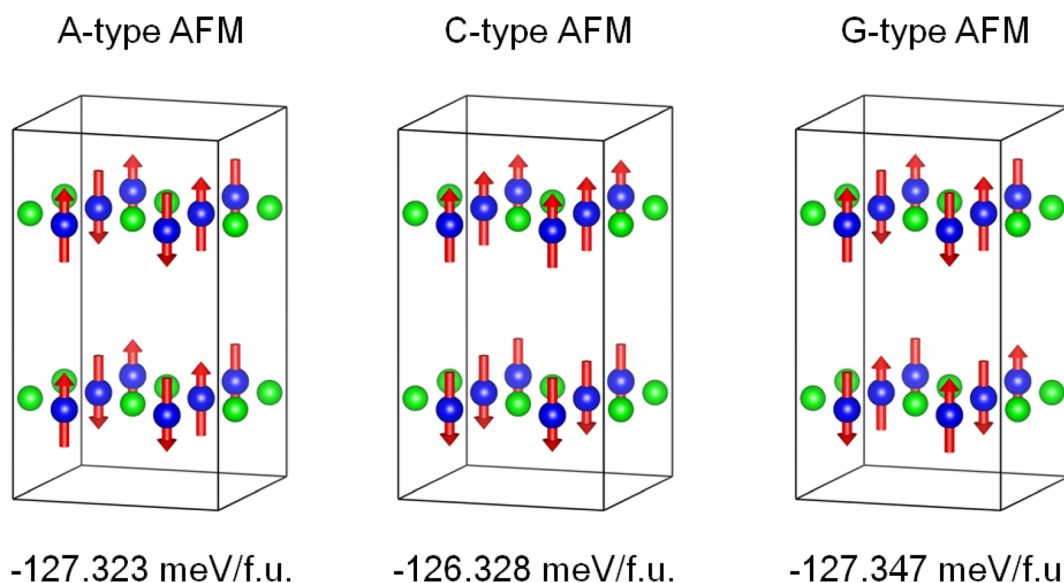
Fig. 5 The calculated energies of different AFM structures of \text{KMnCuTe}_2 in a 2 \times 2 \times 1 supercell, showing that the G-type AFM is the energy favorable ground state of \text{KMnCuTe}_2 .
