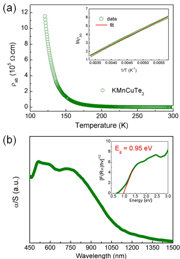
Fig. 4 (a) Temperature dependence of the in-plane resistivity for \text{KMnCuTe}_2 single crystal from 300 to 120 K. Inset shows the fitted result for the data in high temperature range from 300 to 150 K using the thermal activation model. (b) UV-vis diffuse reflectance spectrum of \text{KMnCuTe}_2 . Inset shows the extracted indirect band gap according to Tauc plot.
