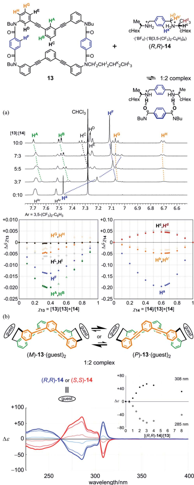
Fig. 7 Complexation of model macrocycle 13 with chiral guests ( R,R )- 14 or ( S,S )- 14 : (a) partial ^1\text{H} NMR spectra of 13 in the presence of ( R,R )- 14 [ [\text{13}] : [\text{14}] = 0 : 10 ( 14 only), 3 : 7, 5 : 5, 7 : 3 and 10 : 0 ( 13 only)], and Job plots ( [\text{13}] + [(\text{R,R})\text{-14}] = 2 \text{ mM} , measured in 3 : 97 (v/v) acetonitrile- d_3 /chloroform- d at 303 K); (b) CD spectra of 13 ( 1.3 \times 10^{-4} \text{ M} ) in the presence of ( R,R )- 14 (blue lines: 1, 2 and 3 equiv.) or ( S,S )- 14 (red lines), measured in dichloromethane at 293 K [inset: plots of induced molar CD versus equivalents of guest added].
