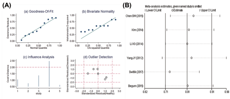
Figure 8. The results of sensitivity analysis (A) Diagnostic value; (B) prognostic value.
