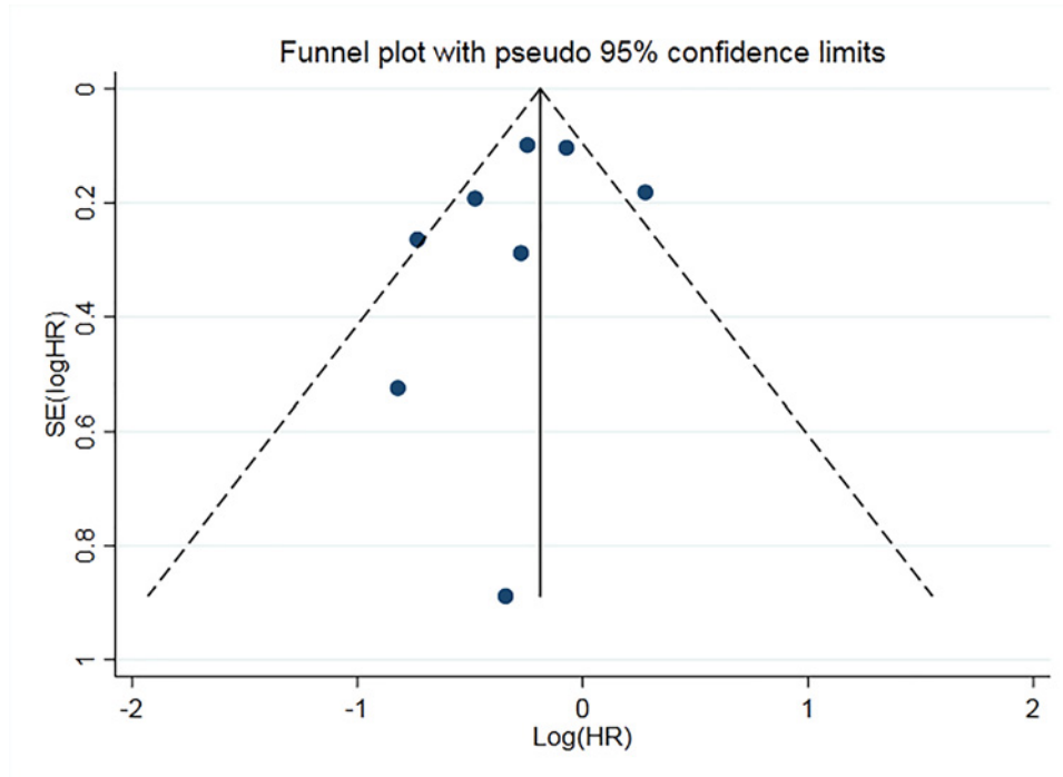
Figure 7. Funnel plot of miR-126 for the prognosis (OS) of NSCLC Abbreviation: SE, standard error.
