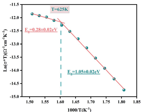
Fig. 8 Arrhenius relation of \text{Ln}(\sigma_{\text{dc}} T) versus 1000/T for the \text{Li}_2\text{CoGeO}_4 compound.
