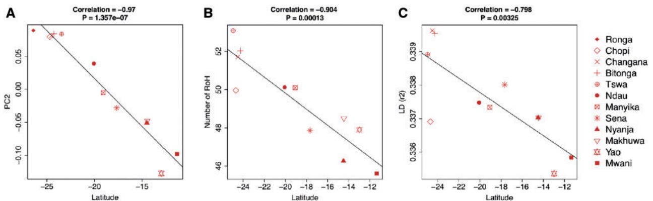
FIG. 2. Genetic variation and geography in Mozambique. The plots show the correlations between latitude and (A) average PC2 scores ( supplementary fig. 1B, Supplementary Material online ) (B) average number of RoHs, and (C) average LD ( r^2 ). In B and C, Tswa and Ronga were lumped and are identified by the Tswa symbol (see supplementary material, Supplementary Material online ).
