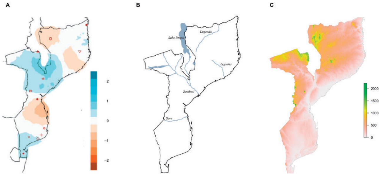
FIG. 3. Estimated Effective Migration Surface (EEMS) analysis. See figure 1 for legend of population symbols. (A) EEMS estimated with 12 Mozambican populations. (B, C) Major rivers (B) and mountains (C) associated with barriers and corridors of migration. The effective migration rates are presented in a log10 scale: white indicates the mean expected rate in the data set; blue and brown indicate migration rates that are X-fold higher or lower than average, respectively. The orographic map (C) was generated with the raster package (Hijmans and van Etten 2011). Altitude is given in meters.
