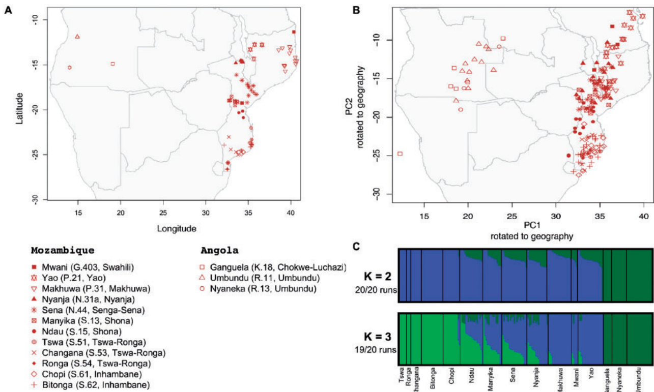
FIG. 1. Genetic structure in Angolan and Mozambican populations. (A) Geographic locations of sampled individuals. The geographic subgroups of Bantu languages (“Guthrie zones”) following Maho (Maho 2003) are given in parentheses in the legend. (B) Principal components 1 and 2 of Angolan and Mozambican individuals rotated to fit geography (Procrustes correlation: 0.89; P < 0.001 ). (C) Population structure estimated with ADMIXTURE assuming 2 and 3 clusters ( K ). Vertical lines represent the estimated proportion of each individual’s genotypes that are derived from the assumed genetic clusters (note that the order of individuals in K = 2 is not the same as K = 3 ). The lowest cross-validation error (CV) was associated with K = 2 (CV values are reported in supplementary table 2, Supplementary Material online ).
