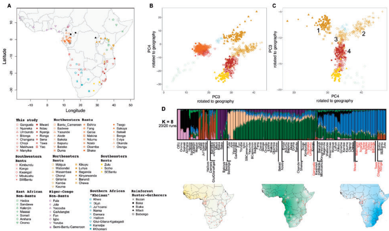
FIG. 4. Genetic structure in African populations. (A) Geographic locations of sampled populations. (B, C) PC plots rotated to geography using Procrustes analysis. (B) All Bantu-speaking populations (Procrustes correlation: 0.76; P < 0.001 ). (C) Only East Bantu-speaking populations (Procrustes correlation: 0.44; P < 0.001 ). The numbers in (C) refer to groups of populations that are discussed in the text. Additional PCA and ADMIXTURE plots are shown in supplementary figures 6 and 8, Supplementary Material online . (D) Population structure estimated with ADMIXTURE assuming eight clusters ( K = 8 ), with Mozambican and Angolan groups from this study labeled in red. Vertical lines represent the estimated proportions of each individual's genotypes that are derived from the assumed genetic clusters (CV values are reported in supplementary table 2, Supplementary Material online ). The maps, obtained by interpolation, display the mean proportions of major ADMIXTURE components ( K = 8 ) from Niger-Congo-speaking populations. The colors in the maps match the colors in the ADMIXTURE plot.
