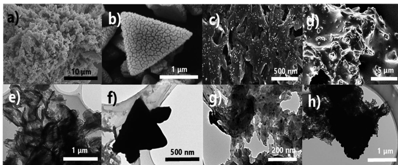
Fig. 2 SEM (a–d) and TEM (e–h) images of (a and e) g\text{-C}_3\text{N}_4 (b and f) \text{Ag}_3\text{PO}_4 , (c and g) UMOFNs, and (d and h) CN10UA.
