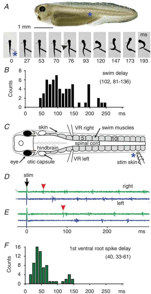
Figure 1. Response times to the first flexion and ventral root burst of swimming to current pulse trunk skin stimulation A, Xenopus tadpole with stimulus site marked (*) and frames from a video (stimulus at t = 0 ms). The tadpole (supported by pins in the neck region) flexes to unstimulated left side starting at 76 ms (arrowhead) and swims off. B, distribution of delays to the start of the 1st flexion of swimming. C, diagram of immobilised tadpole with stimulating and ventral root (VR) recording electrodes. D and E, motor nerve responses to 0.1 ms pulse to trunk skin ( \downarrow ) to show when swimming started on the right, unstimulated side (red arrowheads). F, distribution of delays to the first ventral root spikes when swimming started on the unstimulated side. Numbers in brackets on graphs are median and interquartile range (IQR).
