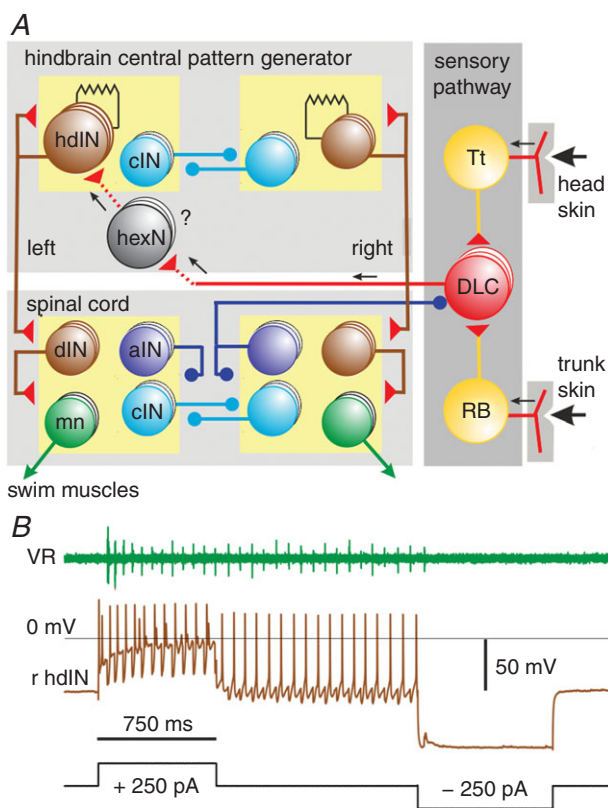
Figure 3. The tadpole swimming network and role of reticulospinal hdIN neurons A, diagram of the touch sensory pathways to the opposite side from the head and trunk skin, and the hindbrain and spinal neurons controlling swimming. Tt, trigeminal touch sensory; RB, Rohon-Beard touch sensory; DLC, dorsolateral commissural sensory pathway; hexN, hindbrain extension neurons; hdIN, hindbrain descending interneurons; cIN, reciprocal inhibitory commissural interneurons; aIN, recurrent inhibitory ascending interneurons; mn, motoneurons. Red triangles are glutamatergic excitatory synapses. Blue circles are glycinergic inhibitory synapses. Synapses onto a box connect to all neurons in the box. B, recording from a right hdIN where activity in the whole swimming network (seen in left ventral root (VR): green trace) could be initiated by positive current and terminated by negative current into this single neuron. The right hindbrain was transected just caudal to the otic capsules (see Fig. 1C).
