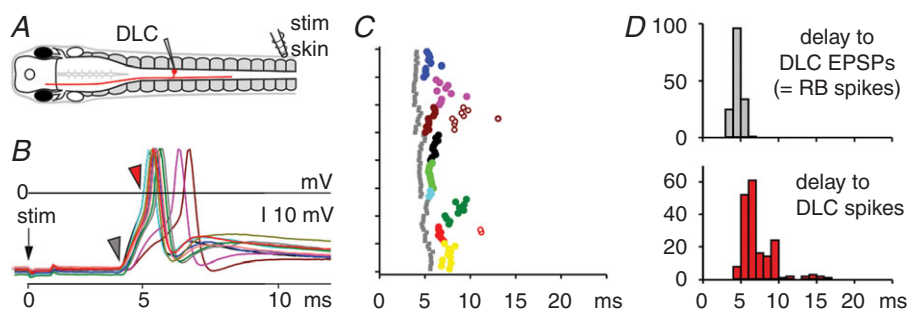
Figure 2. Firing times in sensory pathway DLC neurons following a trunk skin stimulus
