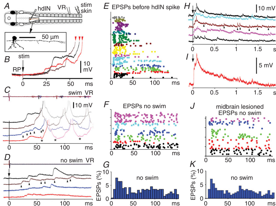
Figure 5. Summation of EPSPs to firing threshold in reticulospinal hdINs following a trunk skin stimulus on the opposite side
