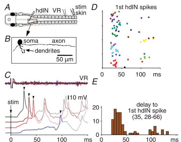
Figure 4. Responses of reticulospinal hdIN neurons to contralateral trunk skin stimulation A, diagram to show the location of electrodes and the recorded hdIN neuron. B, anatomy of hdIN revealed by neurobiotin filling. C, examples of 4 hdIN responses to trunk skin stimulus. Arrowheads mark 1st spike. D and E, hdIN 1st spike time raster plot and 1st spike delays ( n = 80 trials in 13 hdINs).
