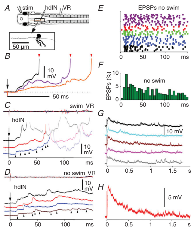
Figure 6. Summation of EPSPs to firing threshold in reticulospinal hdINs following a head skin stimulus on the opposite side
