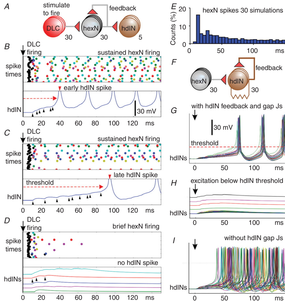
Figure 7. Recurrent models of reticulospinal hdIN excitation and recruitment
