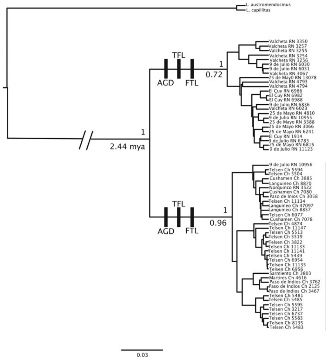
Figure 2. Bayesian phylogram of all unique L. petrophilus haplotypes; numbers above branches are posterior probabilities; numbers below branches are mean estimates of time in millions of years since divergence. Vertical bars represent the three morphological characters (axial groin distance [AGD], third finger lamellae of front limb [TFL], and fourth toe lamellae of hind limb [FTL]) that are significantly different ( P < 0.05 ) between the north and south clades.
