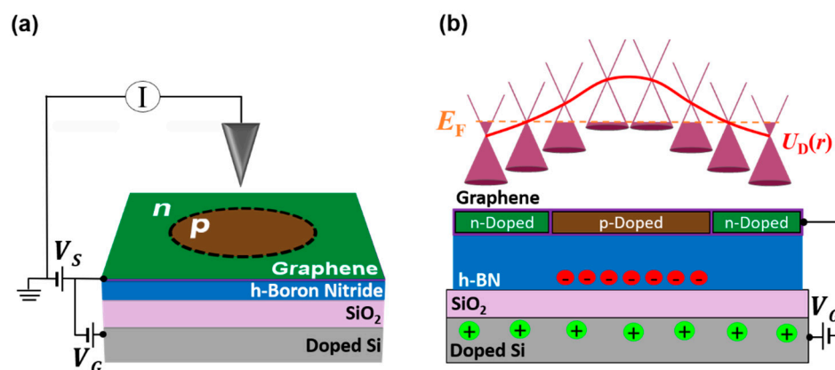
Figure 1. Schematic layout and potential of an exposed graphene Quantum Dot (QD). (a) Schematic showing the scanning tunneling microscope (STM) circuit and graphene/hexagonal boron nitride (hBN) heterostructure. The circular p -doped region outlines the QD created by applying a bias voltage ( V_S ) pulse between the tip and the graphene/hBN heterostructure while holding the back-gate voltage ( V_G ) constant. (b) Top: U_D(r) (red curve) is the potential of the QD which is outlined by tracing along the Dirac point in each cone. Bottom: Side-view schematic of the QD in a graphene/hBN heterostructure for V_G > 0 . The application of a high electric field by the STM tip induces a localized net charge accumulation after exciting defects in hBN. Applying V_G with opposite polarity to charges in hBN induces the spatial variation in doping on graphene which forms the QD boundaries.
