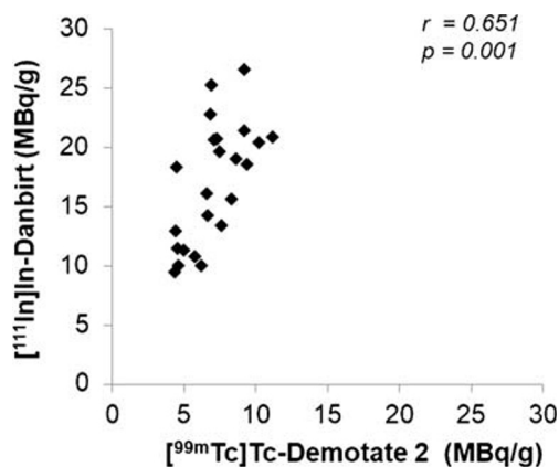
Fig. 6 Positive correlation between [ ^{99m}\text{Tc} ]Tc-Demotate 2 and [ ^{111}\text{In} ]In-Danbirt and in terms of total uptake (MBq/g) per plaque segment
