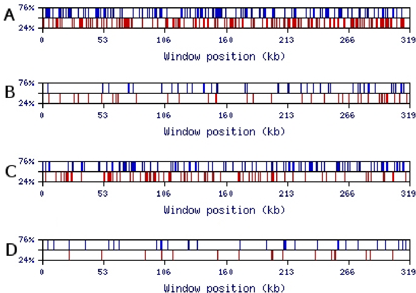
Figure 6 Visualization of MRI-analyzer output for AG- and GT-compositions of 319 kb sequence of the first intron of the DMD gene using a 50 nt window. Upper and lower thresholds are specified on the y-axis as a percentage of the window size. (A) AG-rich and AG-poor regions of the DMD intron; (B) AG-rich and AG-poor regions of the corresponding random SRI-generated set based on the tetramer oligonucleotide frequency table of the DMD intron; (C) GT-rich and GT-poor regions of the DMD intron; (D) GT-rich and GT-poor regions of the corresponding random SRI-generated set based on the tetramer oligonucleotide frequency table of the DMD intron.
