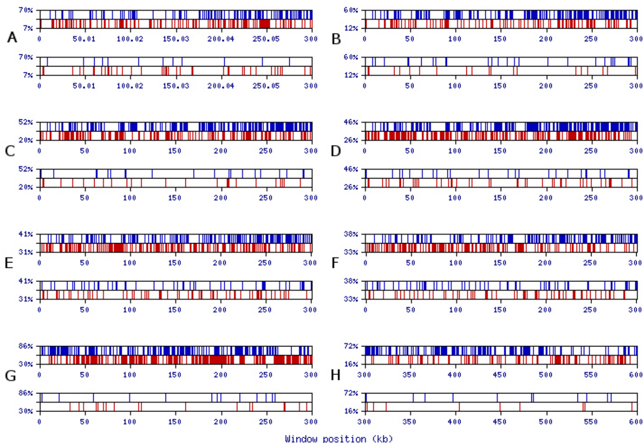
Figure 5 Comparison of MRI-analyses of GC-content for various window sizes and genomic contexts. (A-F) The 319 kb sequence of the first intron from the DMD gene, and its SRI-generated counterpart, analyzed for optimal visual contrast over a range of window sizes (30, 50, 100, 200, 500, 1000) (cf. Figures 4 and 7); (G) The first 300 kb of a sample of human 5'-UTRs and its SRI-generated counterpart using a window size of 50 nt; (H) The 300 kb subset from a sample of intergenic sequences from human chromosome 17 and a corresponding SRI-generated sequence using a window size of 50 nt.
