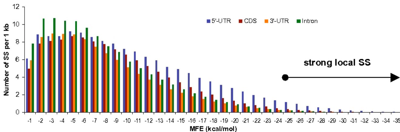
Figure 1 Distribution of local SS with respect to folding energy in mRNA components and introns. Number of structures was measured within 1 kcal/mol intervals and normalized by 1,000 nucleotides of analyzed sequences.
