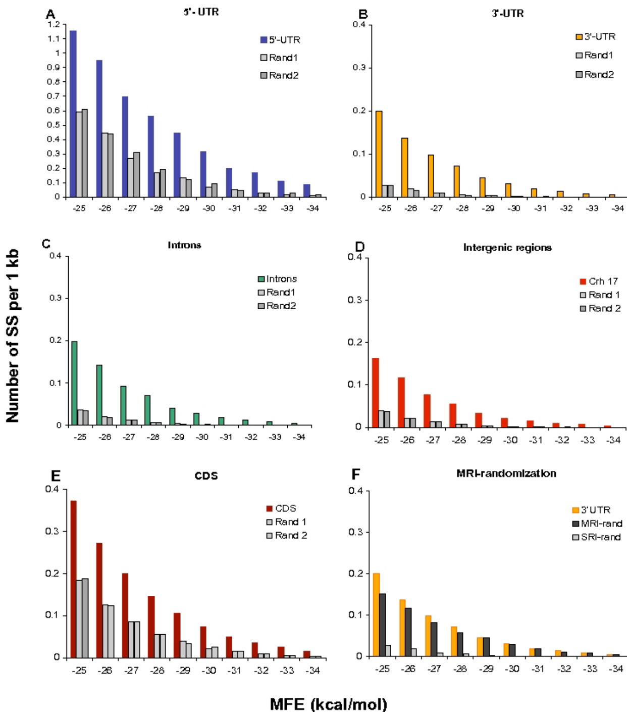
Figure 2 Distribution of strong local SS with respect to folding energy in mRNAs and genomic sequences. Number of structures was measured within 1 kcal/mol intervals and normalized by 1,000 nucleotides of analyzed sequences. (A) 5'-UTRs (blue) and two independent SRI-generated sequences (gray); (B) 3'-UTRs (yellow) and two independent SRI-generated sequences (gray); (C) introns (green) and two independent SRI-generated sequences (gray); (D) intergenic regions from chromosome 17 (red) and two independent SRI-generated sequences (gray); (E) CDS (burgundy) and two independent CDS-generated sequences (gray); (F) 3'-UTRs (yellow), random MRI-generated counterpart sequences (black), and random SRI-generated counterpart sequences (gray).
