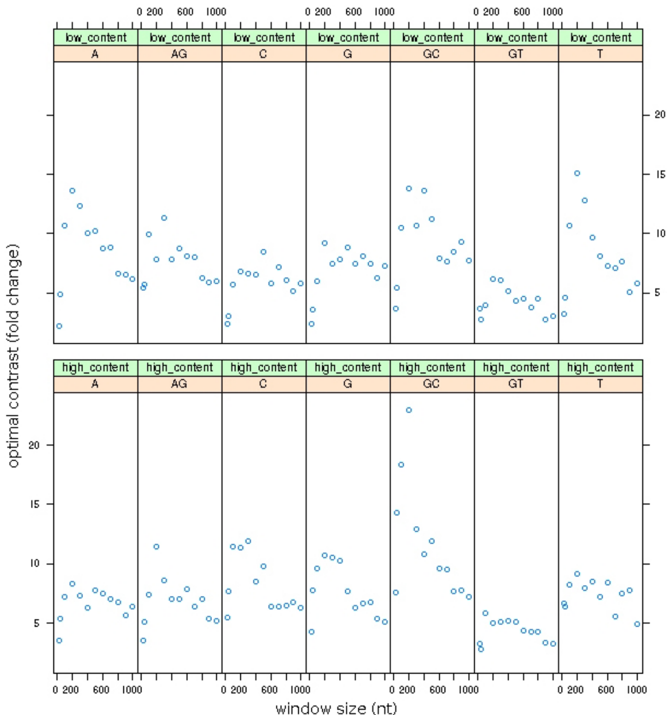
Figure 7 Optimal contrasts for all content types over a range of window sizes. This figure is the "XY conditioning plot" (from the program Rcmdr 1.2) of the optimal contrasts (see text) for regions of high and low content for all seven possible content types over a range of window sizes (30, 50, 100, 200, 300, ... 1000). The sample sequence is the 319 kb first intron from the DMD gene. The SRI-generated counterpart is constructed from the tetramer frequency table derived from the intron.
