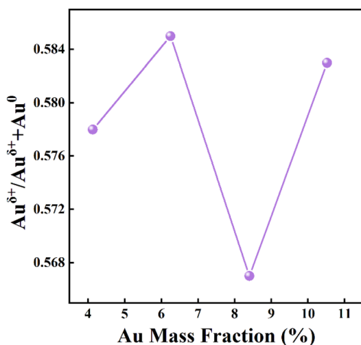
Fig. 6 The influence of Au mass fraction on the \text{Au}^{\delta+}/(\text{Au}^{\delta+} + \text{Au}^0) molar ratio of the \text{Au}_x/\text{Mn}_3\text{O}_4 catalysts.
