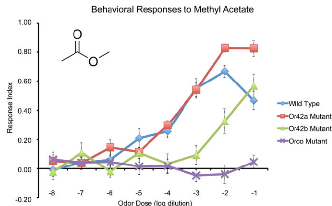
Fig. 3. Behavioral responses of odor receptor mutants to methyl acetate. Inset depicts structural formula of methyl acetate. Error bars represent SEM; n = 10 –16 trials for each point.
