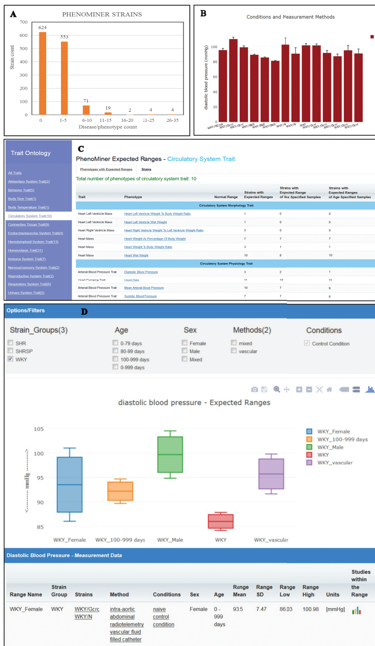
Figure 4. (A) The disease/phenotype annotation distribution of strains with PhenoMiner data. More than half of the PhenoMiner strains have at least one disease/phenotype qualitative annotation. (B) The result page in PhenoMiner after querying WKY strains for diastolic blood pressure, using specific measurement methods under control conditions. The bar chart displays all the matched records in the PhenoMiner database. (C) Summary of the traits for expected ranges analysis is listed on the left and the list of the available expected ranges under the selected circulatory system trait is shown in blue font. Each phenotype is hyperlinked to the associated expected ranges data. (D) The expected ranges of diastolic blood pressure of the selected WKY strain group. Each color-coded box is an interquartile range graph in which the data median is shown as the line in the middle, the third quartile is shown as the top and first quartile is shown as the bottom of the box. Maximum value is represented by the horizontal bar above the box and the minimum value is represented by the horizontal bar below the box. The calculated expected ranges data associated with the displayed graphs are listed at the bottom of the graph, and the links to the original PhenoMiner records are also provided.
