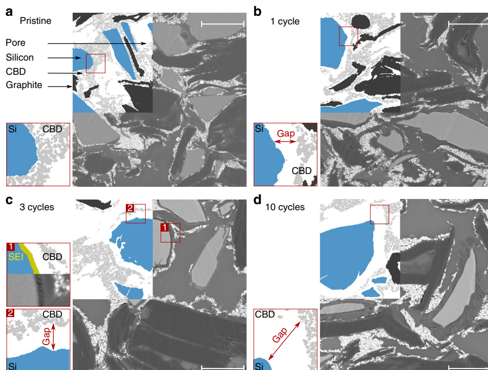
Fig. 3 Scanning electron microscopy. Cross-sectional backscatter scanning electron microscopy images of epoxy infiltrated electrodes in combination with the corresponding multi-phase segmentation for a a pristine electrode and fully delithiated electrodes after b one cycle, c three cycles, and d ten cycles. The red boxes show magnifications at silicon particle surfaces, highlighting the formation and growth of the gap between the silicon particles and the carbon black-binder domain (CBD). The additional inset in c shows that the space between the silicon particles and the carbon black-binder domain is not completely filled with epoxy. Instead, the weakly backscattering dark layer in the vicinity of the silicon particle points to the formation of a thick solid electrolyte interphase (SEI) layer. Scale bars: 5 \mu\text{m}
