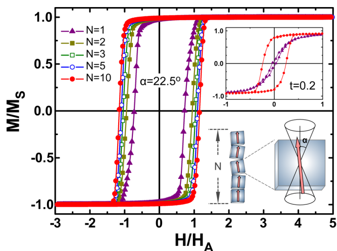
Figure 7 | Chain-like assemblies. Computed hysteresis loops for arrays of nanoparticles of different length (values of N indicated), and the limit case of a single particle, where H_A = 2 K/M_S is the anisotropy field of the particles. The temperature was introduced in terms of the anisotropy energy barrier of the particles, t = k_B T / 2KV = 0.001 . The inset shows the magnetic response on increasing the temperature for the N = 1 and 10 cases, illustrating the higher thermal stability of the chains. The schematic picture shows particles within a chain possessing easy axes contained within an angle of \pi/4 (cubes are only for illustration purposes, since spherical nanoparticles could also form chains).
