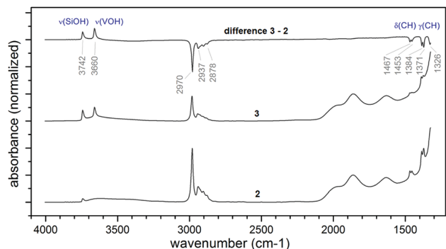
Fig. 1 IR spectra comparing the product of grafting of 1 ( 2 , bottom trace), the material after thermolysis at 200 °C for 1 h ( 3 , middle trace), and the difference spectrum of 2 and 3 (C, top trace).
