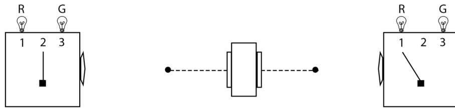
Figure 3. The Mermin device. Alice has her measuring device on the left set to 2 and Bob has his measuring device on the right set to 1. The particles have been emitted by the source in the middle and are in route to the measuring devices.
