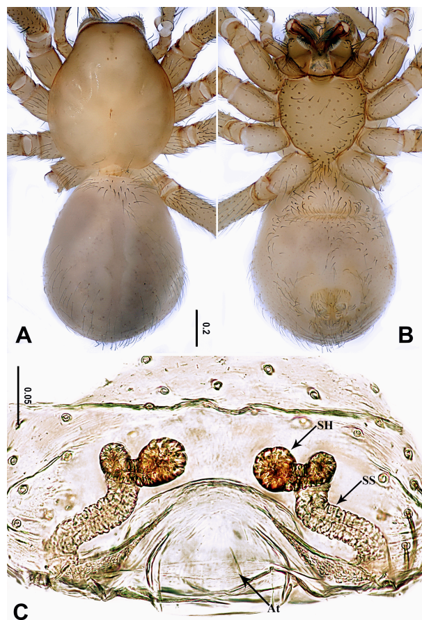
Figure 13 Longileptoneta shenxian sp. nov., female paratype A: Habitus, dorsal view; B: Habitus, ventral view; C: Internal genitalia, dorsal view. At: Atrium; SS: Spermathecae stalk; SH: Spermathecae.
