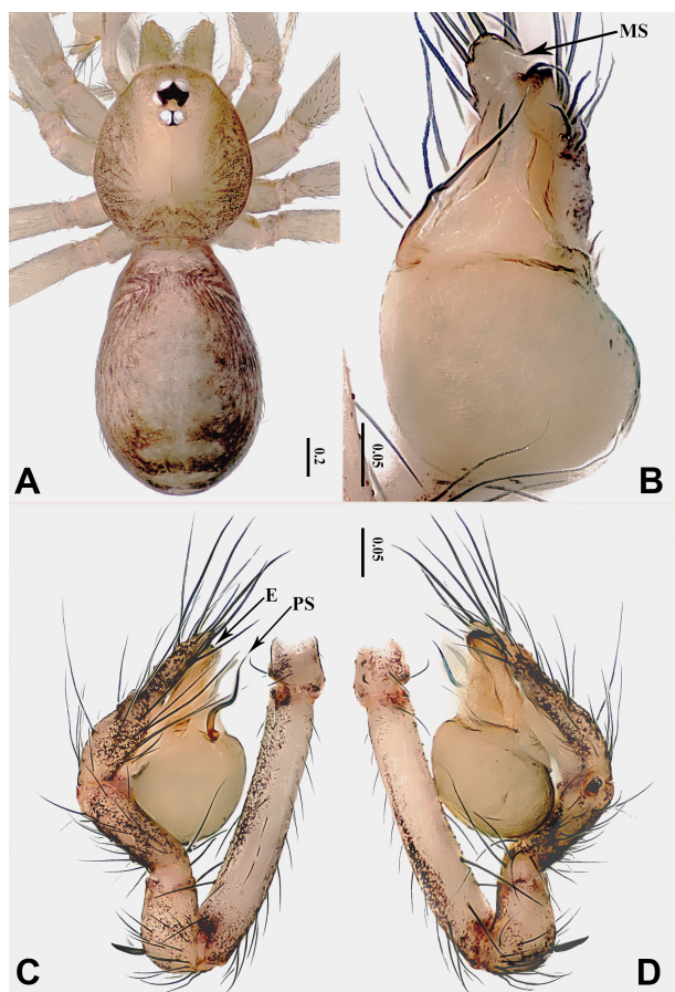
Figure 3 Falcileptoneta shuanglong sp. nov., male holotype A: Habitus, dorsal view; B: Palpal bulb, ventral view; C: Palp, prolateral view; D: Palp, retrolateral view. PS: Prolateral sclerite; E: Embolus; MS: Median sclerite.
