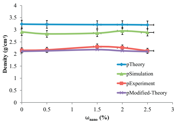
Fig. 1. Density of mixed cement with SONPs versus diverse weight percentages in Theory, Modified-Theory, Experiment and Simulation.
