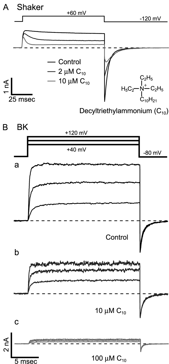
FIGURE 1. No time dependence in the blockage of BK currents by \text{C}_{10} . (A) Time-dependent block of Shaker \text{K}^+ channels by \text{C}_{10} . Macroscopic \text{K}^+ currents were recorded from an inside-out patch from an oocyte expressing Shaker B \Delta 6-46 channels. Under voltage clamp, currents were elicited by depolarization of the membrane potential to 60 mV from a holding potential at -120 mV. Application of 2 \mu\text{M} (dark gray trace) and 10 \mu\text{M} \text{C}_{10} (light gray trace) resulted in reductions of current from the control level (black trace). (B) Macroscopic \text{K}^+ currents carried by BK channels and their responses to \text{C}_{10} . Currents were recorded under voltage clamp from an inside-out patch from an oocyte expressing mslo BK channels. Currents were elicited by depolarizations of the mem-
