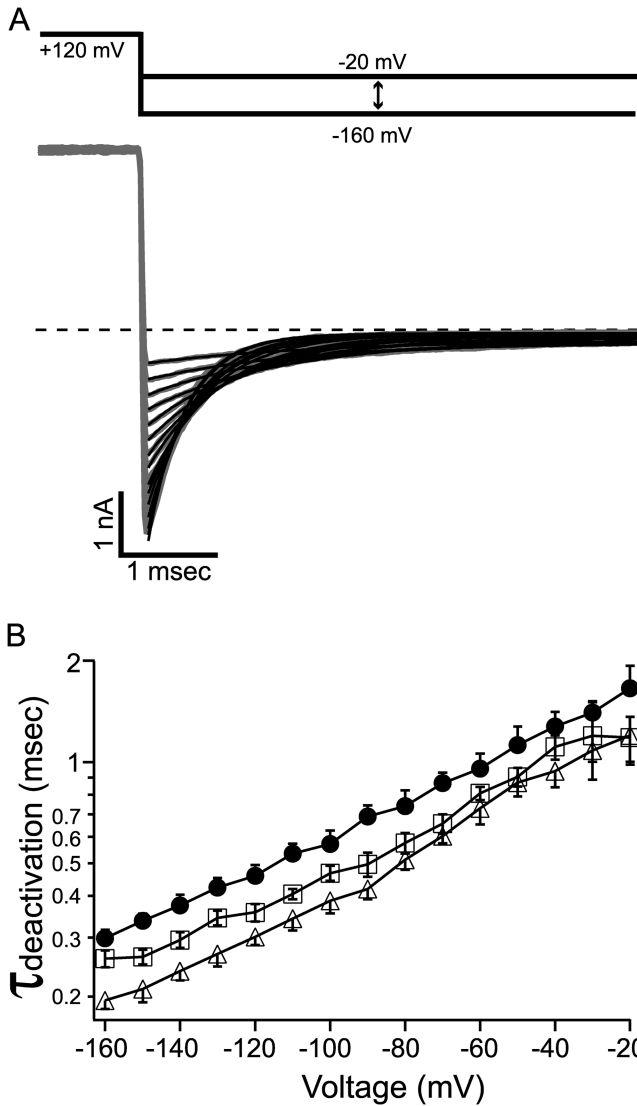
FIGURE 6. Deactivation of BK channel was speeded by C_{10} at all negative membrane potentials. (A) Macroscopic BK currents (gray traces) were recorded from an inside-out patch under voltage clamp. Membrane potential was first depolarized to 120 mV to open all the channels then repolarized to various levels between -160 and -20 mV at 10-mV steps. Tail currents at each potential were fitted with single exponential function (black lines). Tail currents in the presence of 10 or 100 \mu\text{M} C_{10} (not depicted) can also be well fitted with single exponential functions at all negative potentials. (B) Deactivation time constants as measured in A are shown for control (filled circles), 10 \mu\text{M} C_{10} (open squares), and 100 \mu\text{M} C_{10} (open triangles). Each point represents the mean and SEM determined from 6–8 patches. The measurements of deactivation time constants in the absence and presence of C_{10} are from the same patches. The lines connecting the data points have no physical meanings.
