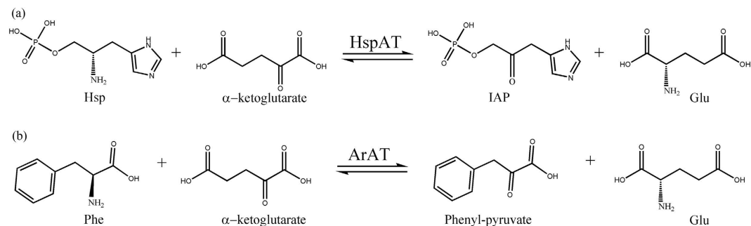
Figure 1. Schematic representation of the biosynthetic steps catalyzed by I \beta aminotransferases. (a) mHspAT catalyzes the reversible conversion of Hsp and imidazole-acetyl phosphate (IAP) and (b) mArAT catalyzes the interconversion of Phe and phenylpyruvate. Both the enzymes use PLP as a cofactor and L-glutamate (Glu) as an amino-donor and convert them into PMP and \alpha -ketoglutarate, respectively.
