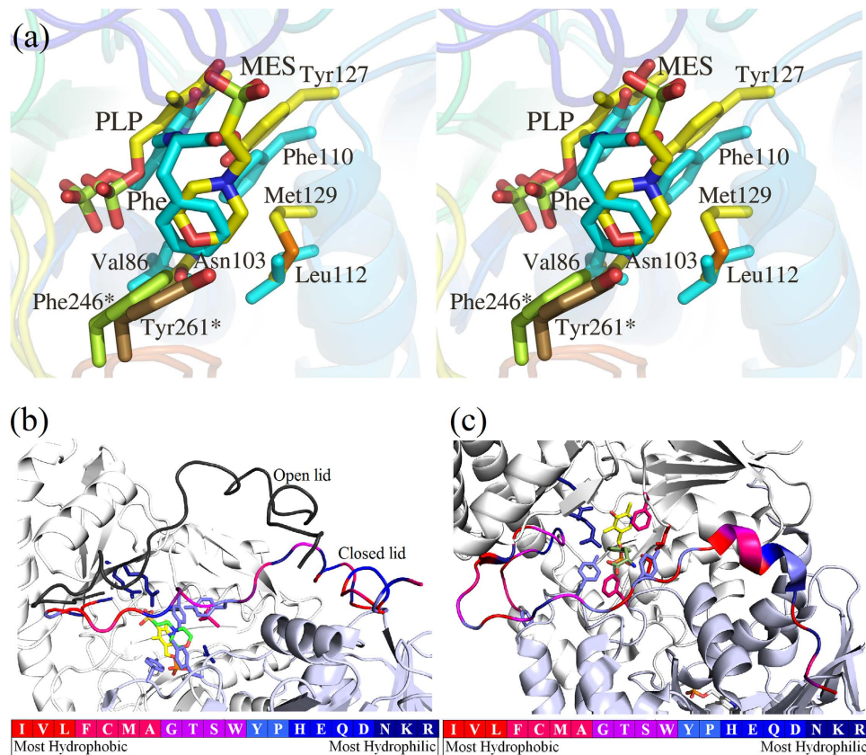
Figure 7. Difference in hydropathicity of residues of mHspAT and mArAT active sites. (a) A stereoview of the superimposition of the active sites of MES- mHspAT and Phe- mArAT complexes shows distinct features. mHspAT possesses a water-loving substrate binding pocket (Asn103, Tyr127, Met129 and Tyr261*) and mArAT harbours a hydrophobic one (Val86, Phe110, Leu112 and Phe246*). Hydropathicity character representations of the N-terminal lid and substrate binding region of (b) mHspAT and (c) mArAT . The hydropathicity index 51 of the individual residues are graphically displayed with the most hydrophobic represented by blue, most hydrophilic represented by red. Substrate binding pockets show a marked difference in the degree of hydropathicity in the two enzymes.
