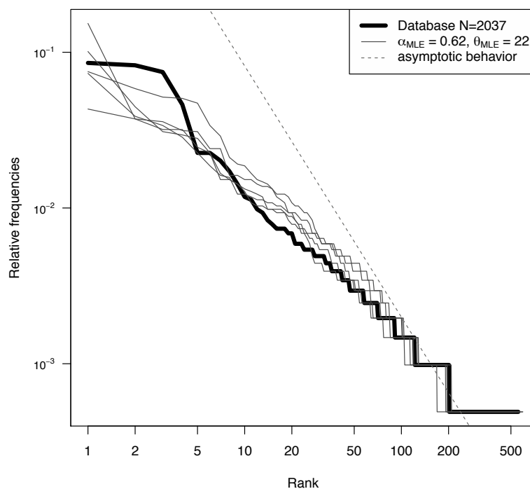
Figure 8. Log scale ranked frequencies from the Dutch database (thick line) compared to the relative frequencies of samples of size n = 2037 obtained from several realizations of \text{PD}(\alpha_{\text{MLE}}, \theta_{\text{MLE}}) (thin lines). Asymptotic power-law behavior is also displayed (dotted line).
