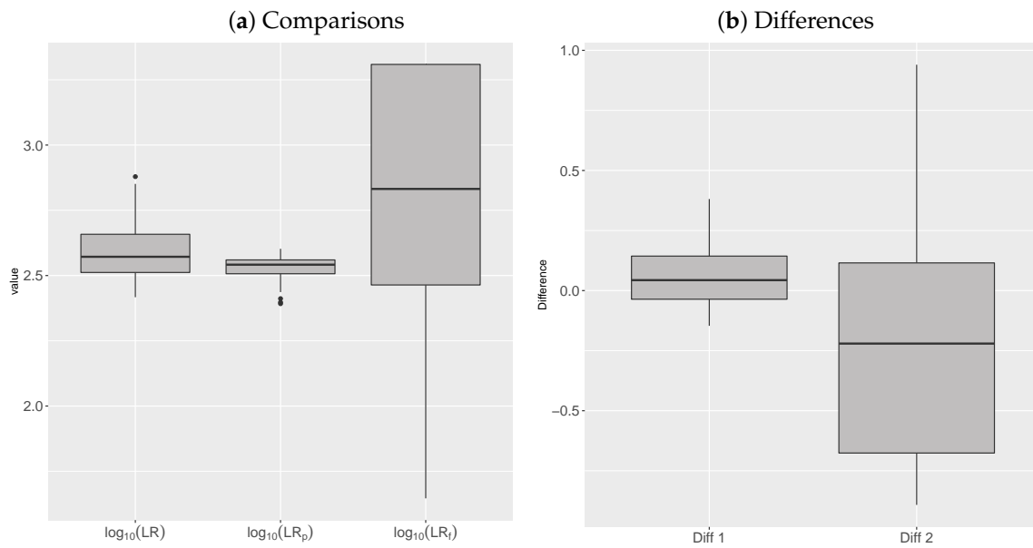
Figure 9. (a) comparison between the distribution of \log_{10} LR , \log_{10} LR_p , and \log_{10} LR_f ; (b) the error \log_{10} LR - \log_{10} LR_p and \log_{10} LR - \log_{10} LR_f .
