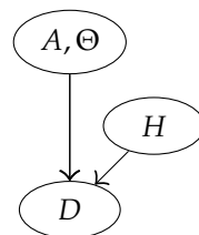
Figure 2. Simplified version of the Bayesian network in Figure 1.
