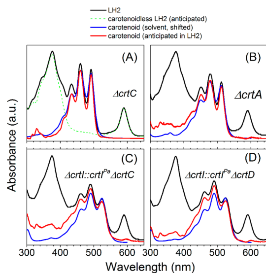
Figure 3. Reconstruction of the carotenoid absorption band in the absorption spectra of the LH2 complexes. The black line represents the LH2 absorption; the blue line is the carotenoid absorption spectrum taken in acetonitrile/THF solvent mixture; the green dashed line is an anticipated absorption spectrum of a carotenoidless LH2. 24 The red profiles are predicted absorption spectra of the carotenoids bound into the LH2s.
