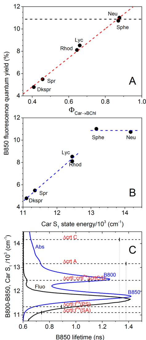
Figure 9. B850 fluorescence quantum yield studies: (A) B850 fluorescence quantum yield as a function \Phi_{\text{Car} \rightarrow \text{BChl}} . (B) B850 fluorescence quantum yield as a function of the carotenoid S 1 ( 2^1\text{A}_g^- ) state energy. (C) Relationship between the B850 fluorescence lifetime, the S 1 ( 2^1\text{A}_g^- ) excited-state energy of the main carotenoid bound in a particular LH2, and the energies of the B800 and B850 bands. The dotted lines in panels (A) and (B) are guides to the eye.
