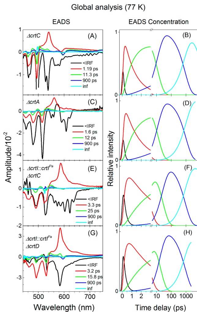
Figure 7. Global analysis results of 77 K TA data sets given in Figure 5. The fitting applied a sequential model of excitation decay path and gives EADS with corresponding decay lifetimes (left column). The contribution of a particular EADS in the raw TA spectrum at a certain delay time is given by the EADS concentration (right column).
