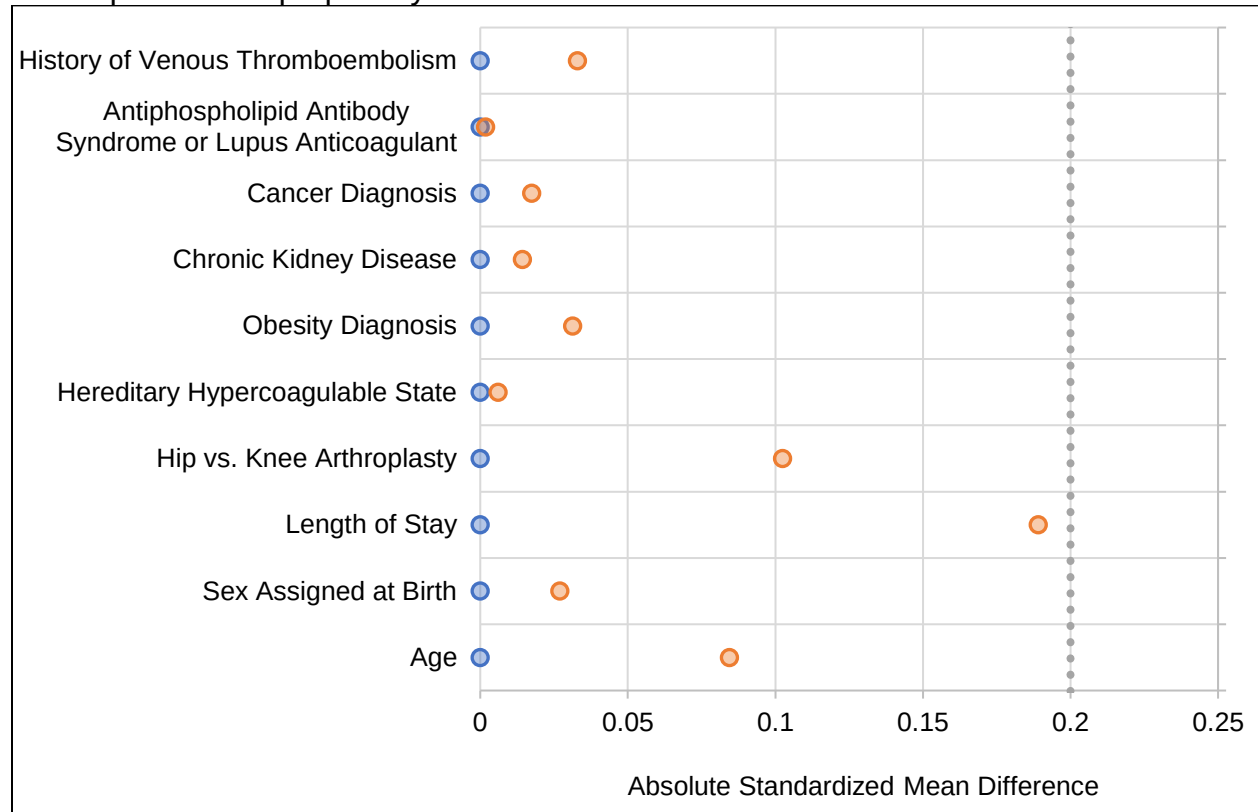
eFigure 2. Absolute standardized mean differences between direct oral anticoagulant and aspirin patients. Orange dots represent the whole cohort and blue dots represent the propensity matched cohort.
