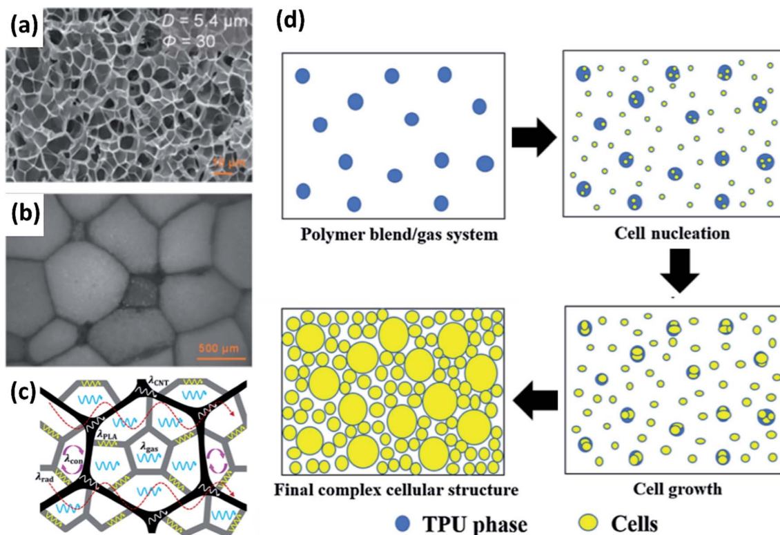
Fig. 5 Examples of PLA foam structures. (a–c) Foamed PLA beads wrapped in a carbon nanotube network reproduced from ref. 24 with permission from American Chemical Society, copyright 2017. (a) SEM micrograph of expanded PLA; (b) sintered expanded PLA beads with CNT network; (c) heat transfer diagram. (d) Schematic of proposed formation process of bimodal cell structure dependent on difference in nitrogen diffusion through the two polymer phases reproduced from ref. 41 with permission from Elsevier, copyright 2019. White areas denote PLA, blue areas denote thermoplastic PU, and yellow denotes a cell. 24,41
