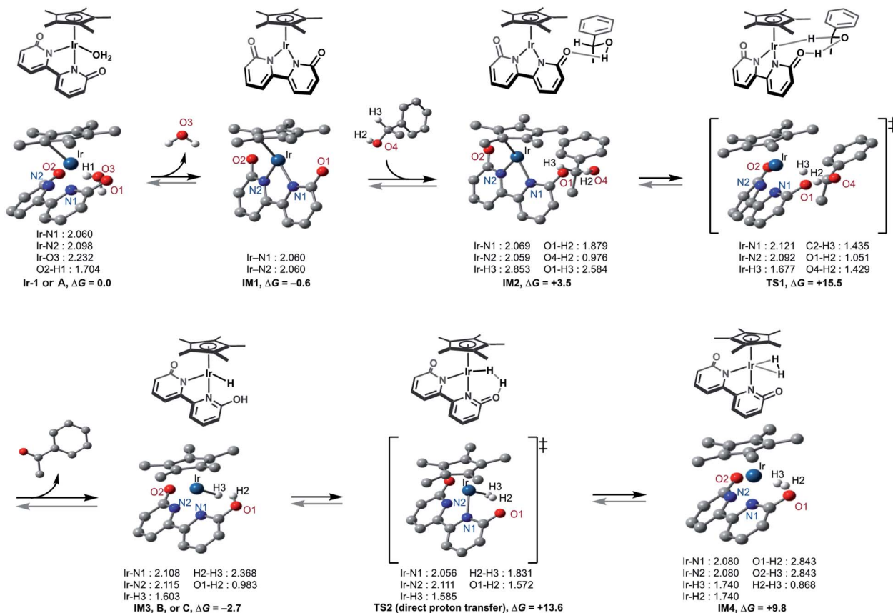
Fig. 5 Geometry and energy changes of the proposed pathway at the CAM-B3LYP + GD3 level of theory using SDD and 6-31+G** basis sets for Ir and other atoms, respectively. Solvent effect (H 2 O) by IEFPCM method; Gibbs free energies in kcal mol -1 at T = 353.15 K.
