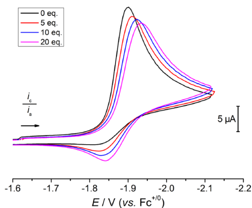
Figure 7. CV of 0.8 mM 1 in THF containing 0.2 M [ n Bu 4 N][PF 6 ] and 0–20 equiv [ n Bu 4 N]Cl under N 2 at 0.1 V·s -1 .
