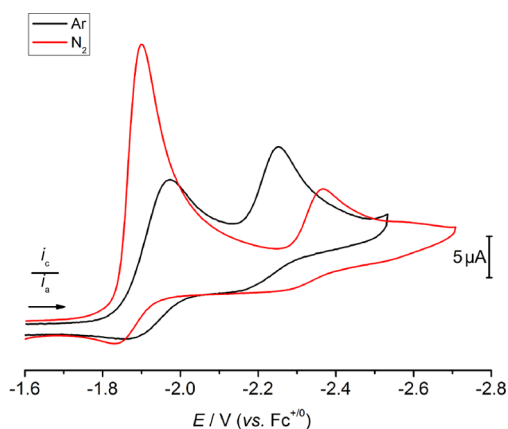
Figure 6. CV data of 1 in THF containing 0.2 M [ n Bu 4 N][PF 6 ] under 1 atm N 2 (red) and Ar (black). Conditions: 1 (0.8 mM) in 0.2 M [ n Bu 4 N][PF 6 ] measured at 0.1 V·s -1 .
