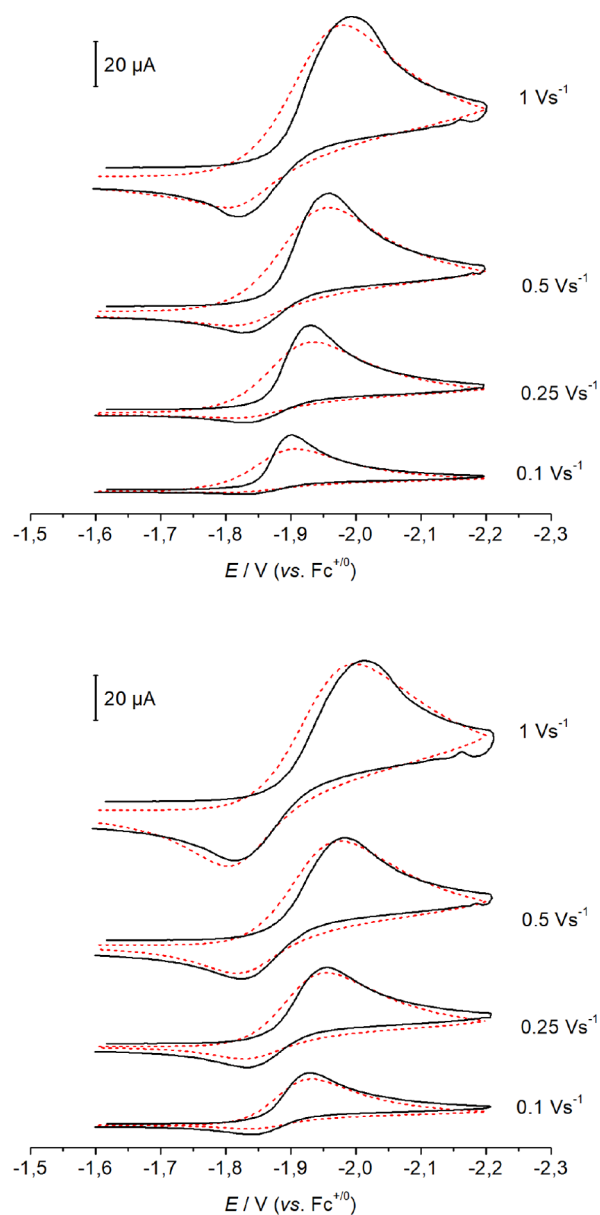
Figure 8. Overlay of experimental (black lines) and simulated (red dashed lines) CV data ( I = 0.2 M [^nBu_4N][PF_6] in THF at room temperature) for 1 (top) and 1 with 10 equiv [^nBu_4N]Cl (bottom). Simulation according to Scheme 5 with the thermodynamic and kinetic parameters given in Tables 1 and 2.
