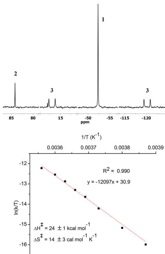
Figure 1. (top) ^{31}\text{P}\{^1\text{H}\} NMR spectrum during reduction of 1 at -30\text{ }^\circ\text{C} under \text{N}_2 . (bottom) Eyring plot for the conversion of 3 to 2 in the temperature range -15 to +7.5\text{ }^\circ\text{C} .
