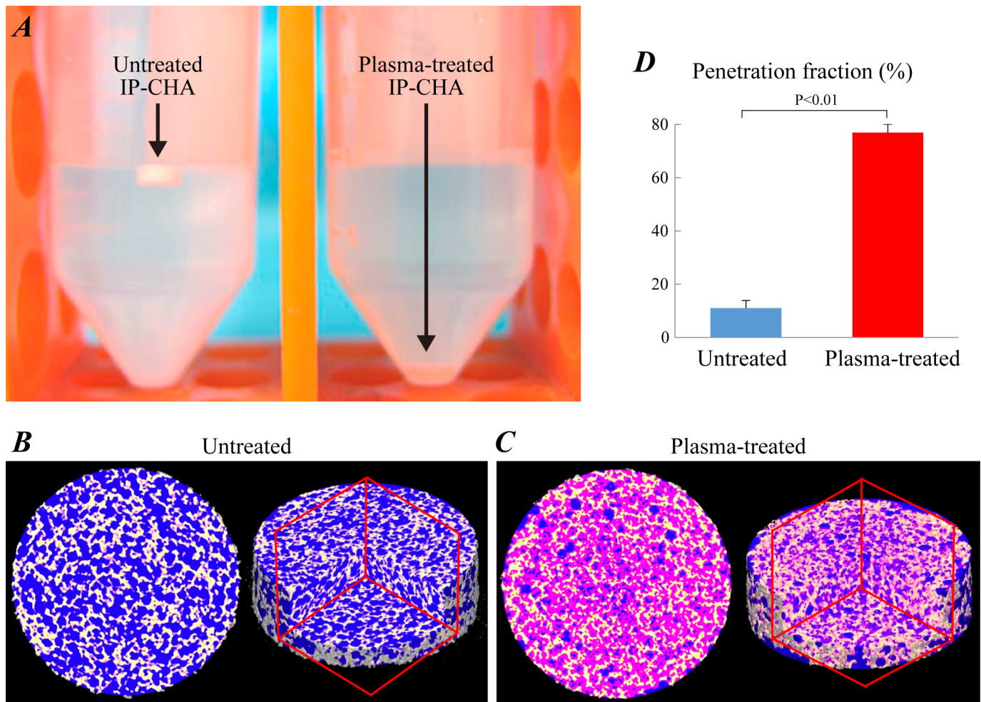
Fig 3. Analysis of water penetration into IP-CHA. (A) Photographs of untreated and plasma-treated IP-CHA discs ( \varphi 5 \text{ mm} \times h 2 \text{ mm} ) soaked in the deionized water containing 6% contrast medium (CM, Oypalomin™). Both discs were soaked in the CM solution for 10 minutes, and evaluated by \mu CT regarding penetration of CM solution into inner pores. The \mu CT cross section at half height (left) and 3D (right) images of untreated (B) and plasma-treated IP-CHA discs (C). Each image is composed of three parts: yellow for HA, blue for empty space (i.e. unfilled pores) and pink for the CM solution (i.e. CM filled pores). (D) Penetration fraction of inner pores was calculated. Data were expressed as mean \pm SD.
