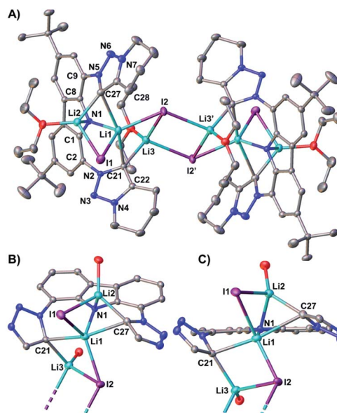
Fig. 4 (A) The molecular structure of dimeric L 5 contains six lithium atoms and four bridging iodo ligands. Thermal ellipsoids are shown at the 50% probability level; hydrogen atoms are omitted for clarity. The monomers are shown from different views in (B) and (C), for which the annulated six-membered rings, t Bu groups, ethyl fragments of the diethyl ether and all hydrogen atoms have been omitted for clarity. Selected bond lengths [Å], angles [°], and dihedral angles [°]: N1–C1 1.3837(19), N1–C8 1.3899(19), C9–N5 1.4302(19), N5–N6 1.3396(18), N6–N7 1.3251(19), N7–C28 1.356(2), C28–C27 1.392(2), C27–N5 1.373(2), C27–Li2 2.136(3), Li2–I1 2.776(3), I1–Li1 2.911(3), Li1–I2 2.748(3), Li1–I1 2.911(3), C27–Li1 2.633(3), Li3–I2' 2.850(3), Li3–I2 2.970(3), C21–Li1 2.391(3), C21–Li3 2.216(3), C21–N2 1.3771(19), N2–N3 1.3414(17), N3–N4 1.3249(18), N4–C22 1.357(2), C22–C21 1.398(2), C2–N2 1.4348(19), N1–Li1 2.052(3), N1–Li2 2.188(3), C1–N1–C8 103.18(12), N2–C21–C22 100.22(12), N5–C27–C28 100.25(13), C1–C2–N2–N3 137.4(1), C8–C9–N5–N6 151.3(1).
