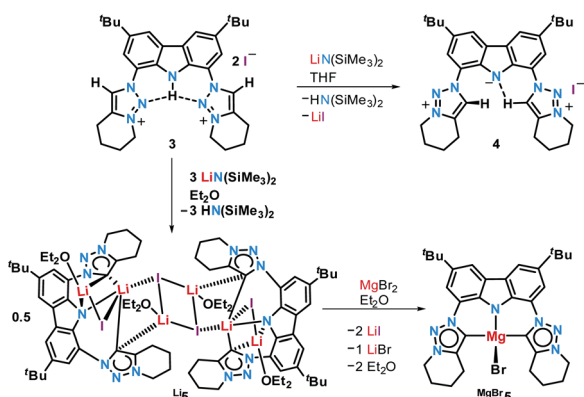
Scheme 2 Deprotonation of 3 to 4 and L 5 and subsequent transmetalation to Mg 5 .
