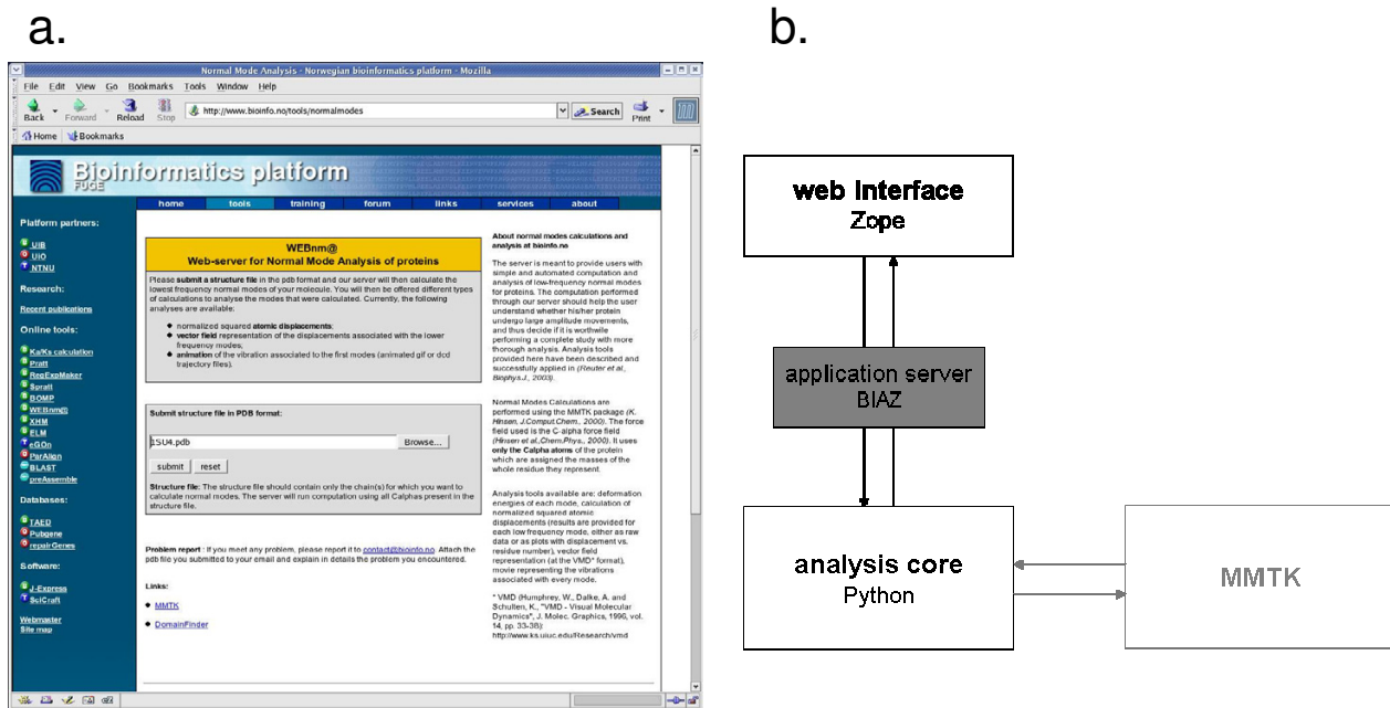
Figure 1 WEBnm@ architecture. a. The main page of WEBnm@ is a form where users can input a structure file in the PDB format. b. The server consists of two parts, the graphical web interface and the core of the program, written in Python, which performs the actual computation. The two parts communicate via a web application server, BIAZ.
