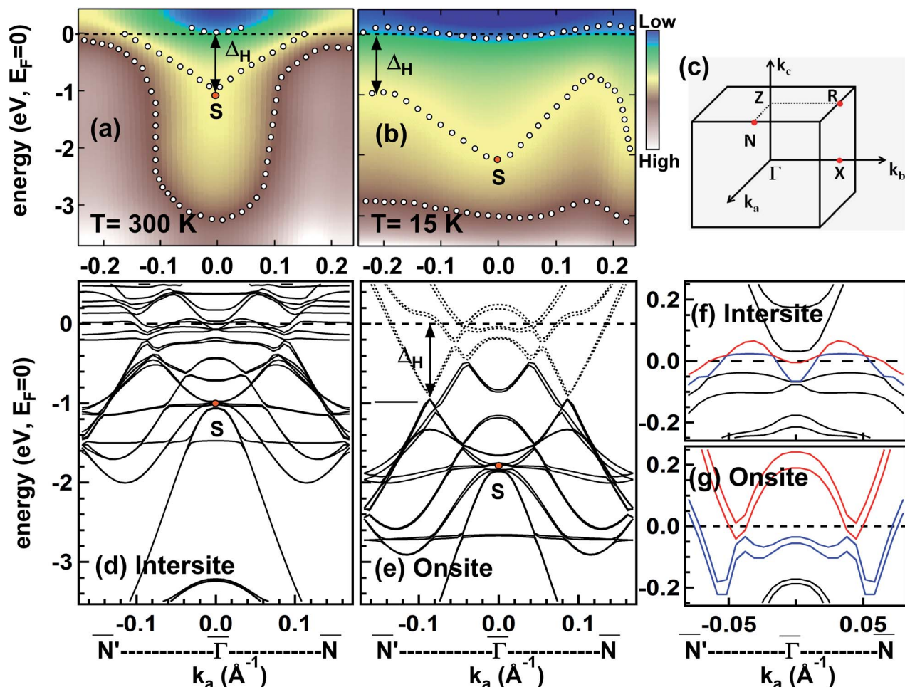
Fig. 4 ARPES band structure along the \bar{N}'-\bar{\Gamma}-\bar{N} direction at (a) RT (300 K) and at (b) LT (15 K) are shown. White dots are the guide to eye for the bands observed and the red dot indicates the van Hove singularity (S). (c) Shows the Brillouin zone with the projected 2D surface which is probed experimentally. Calculated band structures for intersite and onsite bulk calculations are shown in (d) and (e), respectively. A zoomed-in region near E_F for intersite and onsite bulk calculations are shown in (f) and (g), respectively.
