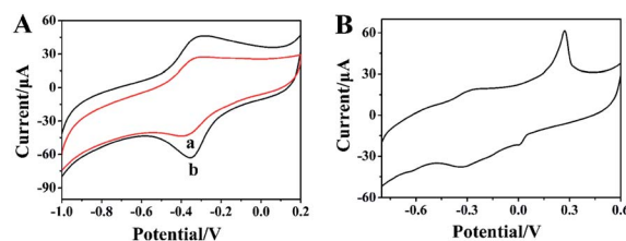
Fig. 3 CVs of rGO-H/GCE (a) and rGO-H-Ag/GCE (b) in \text{N}_2 -saturated 0.2\text{ M pH } 7.0\text{ PB} (A); CVs of rGO-H-Ag/GCE in \text{N}_2 -saturated 0.2\text{ M pH } 7.0\text{ PB} (B). Scan rate: 100\text{ mV s}^{-1} .
