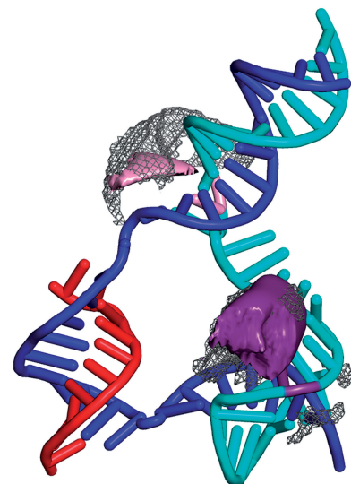
Figure 3. Consistency check of built model. A 38% credibility volume for dye molecule attached to nontemplate DNA at register -2 (purple) and -12 (pink) determined using NPS (surface representation) and computed accessible volume for a dye molecule attached to the respective position of the modeled nontemplate DNA (gray meshes).
