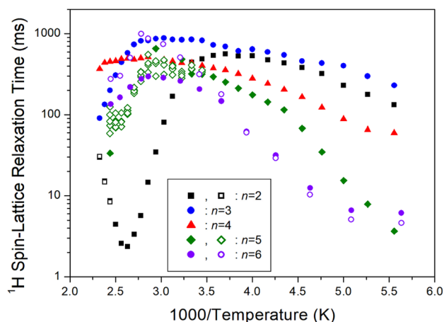
Fig. 11 ^1\text{H} spin-lattice relaxation times T_{1\rho} of [\text{NH}_3(\text{CH}_2)_n\text{NH}_3]\text{ZnCl}_4 ( n = 2, 3, 4, 5, and 6 ) for various methylene chain lengths as a function of 1000/\text{temperature} .
