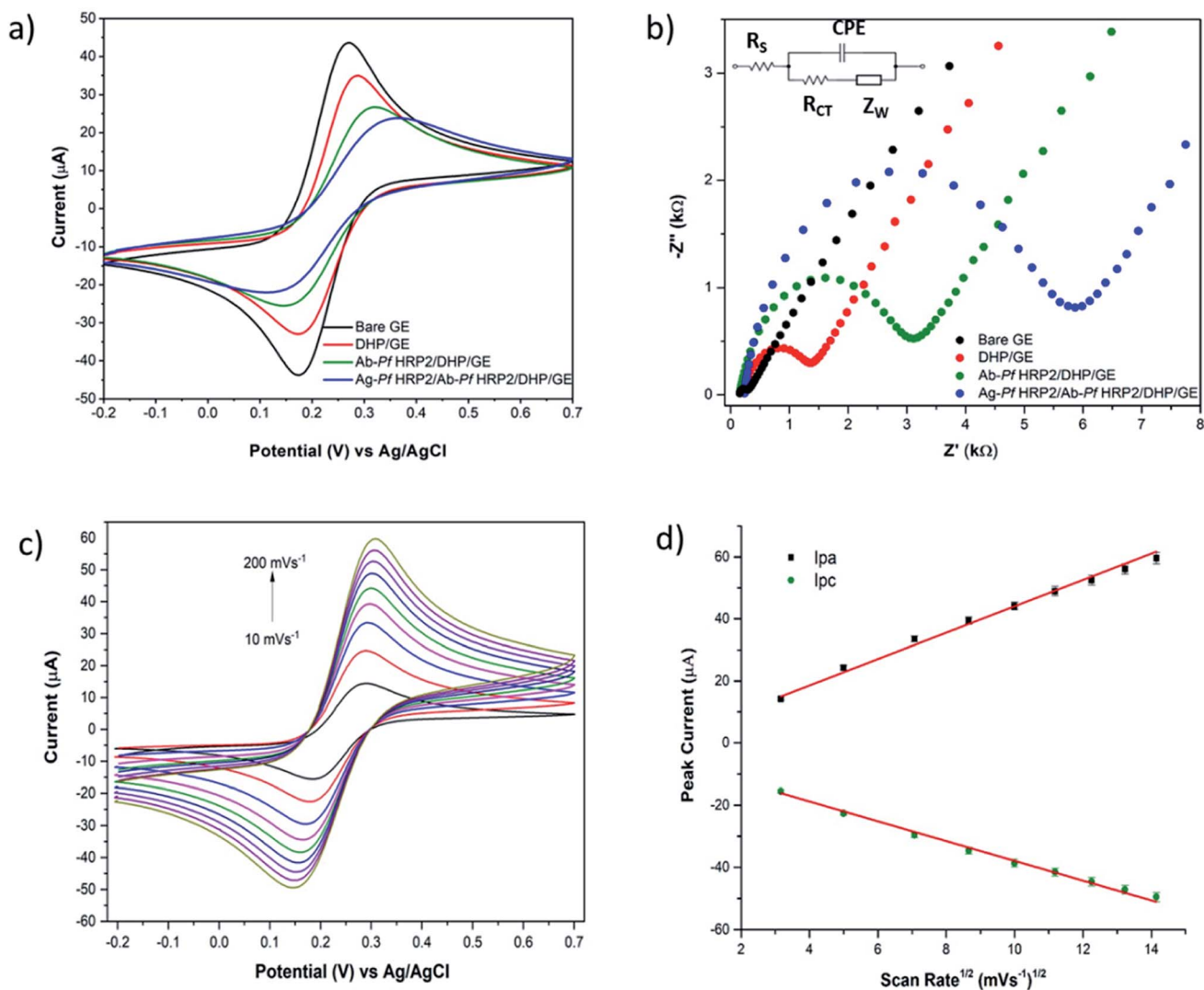
Fig. 3 (a) CVs recorded between -0.2 and +0.7 V at 50 \text{ mV s}^{-1} , (b) EIS recorded at +0.23 V by varying the frequency with logarithmic spacing frequency in the range from 10 mHz to 100 kHz, (c) CVs recorded with the immunosensor at different scan rates ( 10, 25, 50, 75, 100, 125, 150, 175, 200 \text{ mV s}^{-1} ), and (d) plots of peak currents as a function of the square root of the scan rate. All the electrochemical measurements were carried out in 5 \text{ mmol L}^{-1} [\text{Fe}(\text{CN})_6]^{4-/3-} + 0.1 \text{ mol L}^{-1} \text{ KCl} solution.
