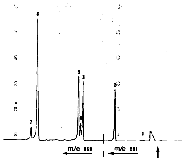
FIGURE 6 Mass fragmentogram of the sugar derivatives of the hydrolysate of fetuin prepared by PAGE ( 40 \mu\text{g} of protein recovered, 2 \mu\text{g} of internal standard added; for further explanation, see Fig. 3). The asymmetric artifact peak near the region where fucose is normally detected is consistently observed and is derived from acrylamide acetate from the gel; however, it does not interfere with determination of fucose (7).
