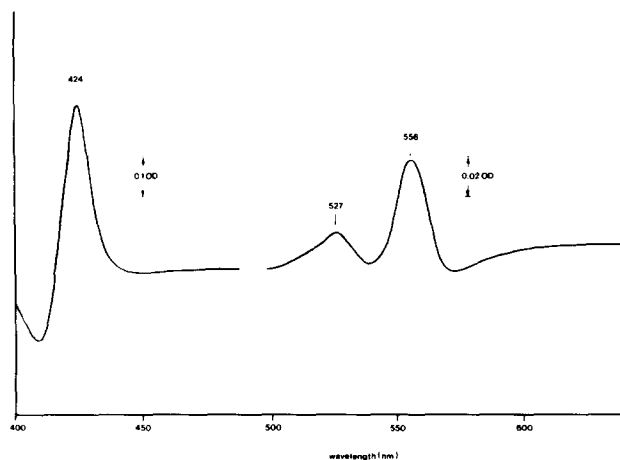
FIGURE 1 Difference spectrum of purified tryptic fragment of cytochrome b_5 . Dithionite-reduced vs. oxidized protein was recorded at room temperature. Optical path was 1 cm and band width 3 mm. For further details, see reference 19.
