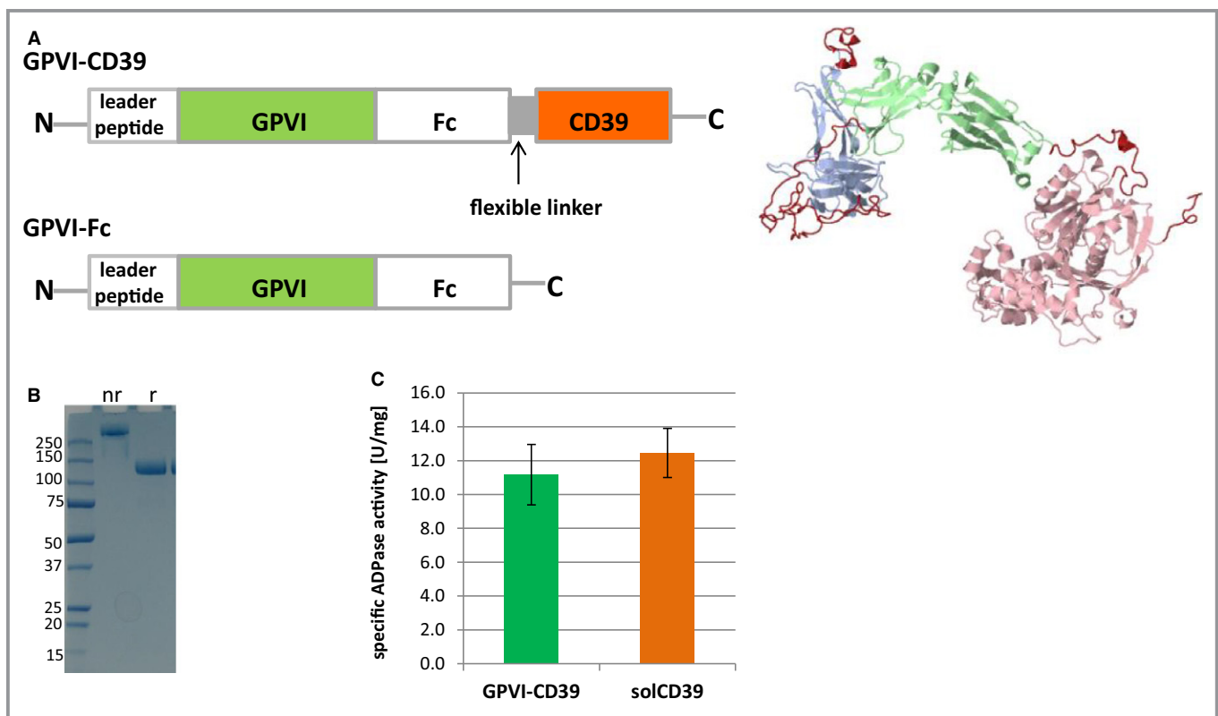
Figure 1. Structure scheme and biochemical characterization of bifunctional, recombinant GPVI-CD39 compared to GPVI-Fc. A, Structure (left panel) and putative 3D-modeling (right panel) of bifunctional, recombinant GPVI-CD39 compared with GPVI-Fc. The 3D model shows the extracellular GPVI domains in blue, the Fc part in green, and the CD39 domain in light red. The N-terminal leader peptides of each protein are cleaved before secretion of each protein. B, Coomassie staining of GPVI-CD39 as purified from supernatants of GPVI-CD39-expressing cells. C, Specific ADPase activity of recombinant GPVI-CD39 (333 nmol/L) in comparison to that of commercially available soluble CD39 (666 nmol/L; n=3, mean \pm SEM). Both specific activities were determined at other enzyme molarities and did not differ, as expected, because substrate concentrations were not limiting. GPVI indicates glycoprotein VI; GPVI-CD39, dimeric glycoprotein VI and CD39 fusion protein; GPVI-Fc, dimeric glycoprotein VI; nr, nonreducing conditions; r, reducing conditions.
