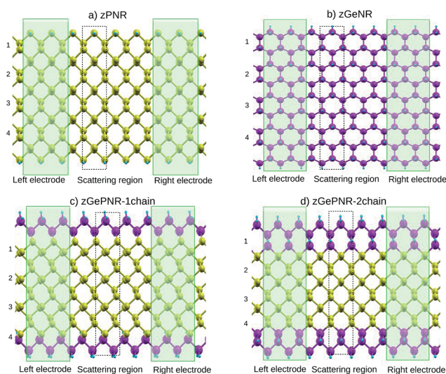
Fig. 1 Schematic representation of (a) zPNR, (b) zGeNR, (c) zGePNR-1chain and (d) zGePNR-2chain. The green rectangles denote the semi-infinite left and right electrodes. One unit cell in the scattering region is indicated by a dashed rectangle. The numbers listed on the left side of the computational models indicate the width of the nanoribbons. Phosphorus, germanium and hydrogen are represented by yellow, purple and blue spheres, respectively.
